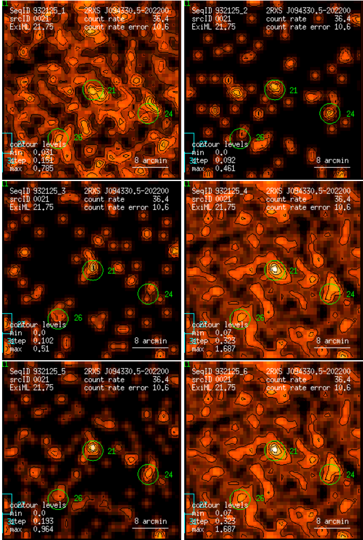
Figure 21: RASS 932125: detection 0021: band rate images, Gaussian filter: (1) PSPC channels 11 – 41, (2) 52 – 90, (3) 91 – 201, (4) 11 – 235, (5) 52 – 201, (6) 11 – 201. Broad band rates in counts/ks. Band rate contour levels in counts/ks/arcmin 2 .
