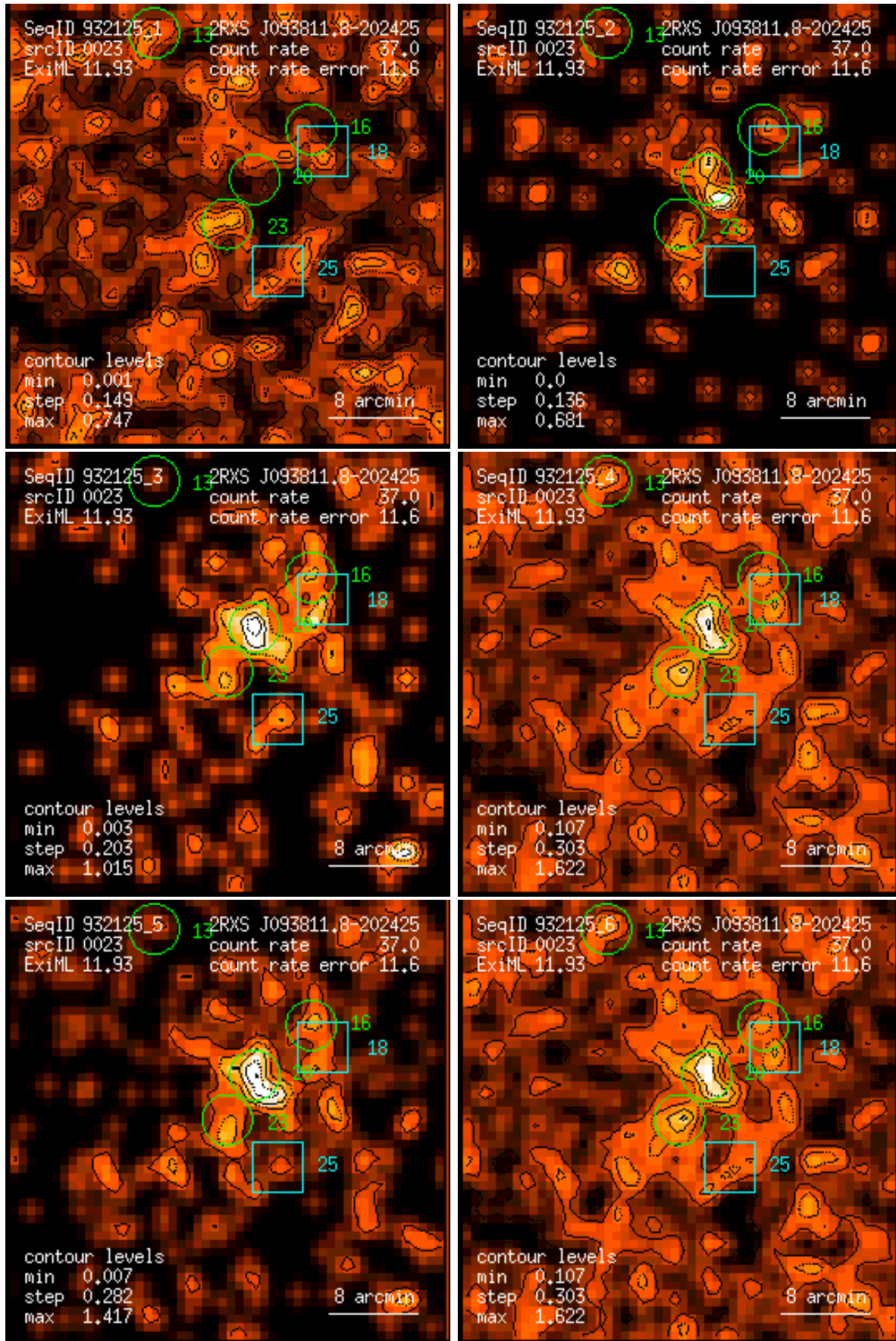
Figure 23: RASS 932125: detection 0023: band rate images, Gaussian filter: (1) PSPC channels 11 – 41, (2) 52 – 90, (3) 91 – 201, (4) 11 – 235, (5) 52 – 201, (6) 11 – 201. Broad band rates in counts/ks. Band rate contour levels in counts/ks/arcmin 2 .
