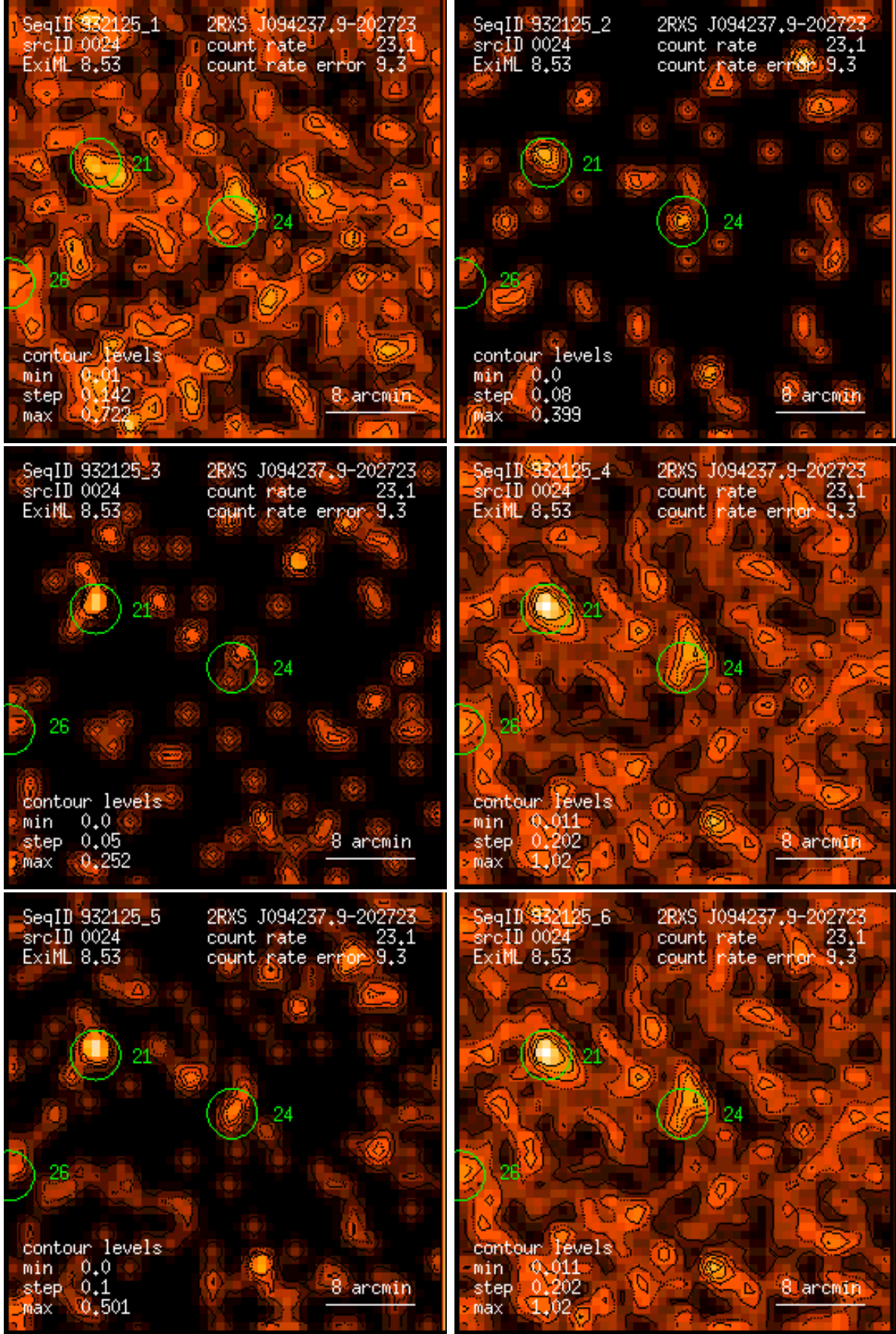
Figure 24: RASS 932125: detection 0024: band rate images, Gaussian filter: (1) PSPC channels 11 – 41, (2) 52 – 90, (3) 91 – 201, (4) 11 – 235, (5) 52 – 201, (6) 11 – 201. Broad band rates in counts/ks. Band rate contour levels in counts/ks/arcmin 2 .
