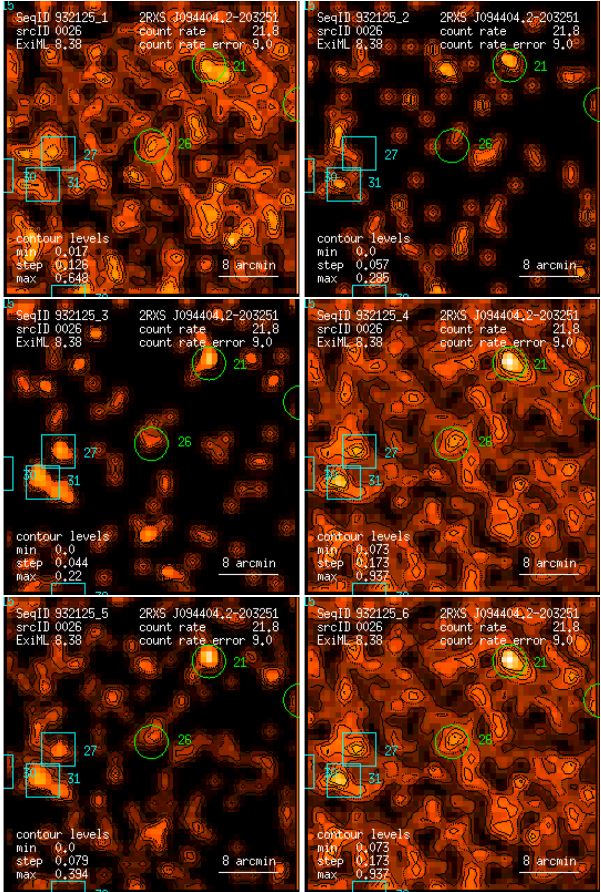
Figure 26: RASS 932125: detection 0026: band rate images, Gaussian filter: (1) PSPC channels 11 – 41, (2) 52 – 90, (3) 91 – 201, (4) 11 – 235, (5) 52 – 201, (6) 11 – 201. Broad band rates in counts/ks. Band rate contour levels in counts/ks/arcmin 2 .
