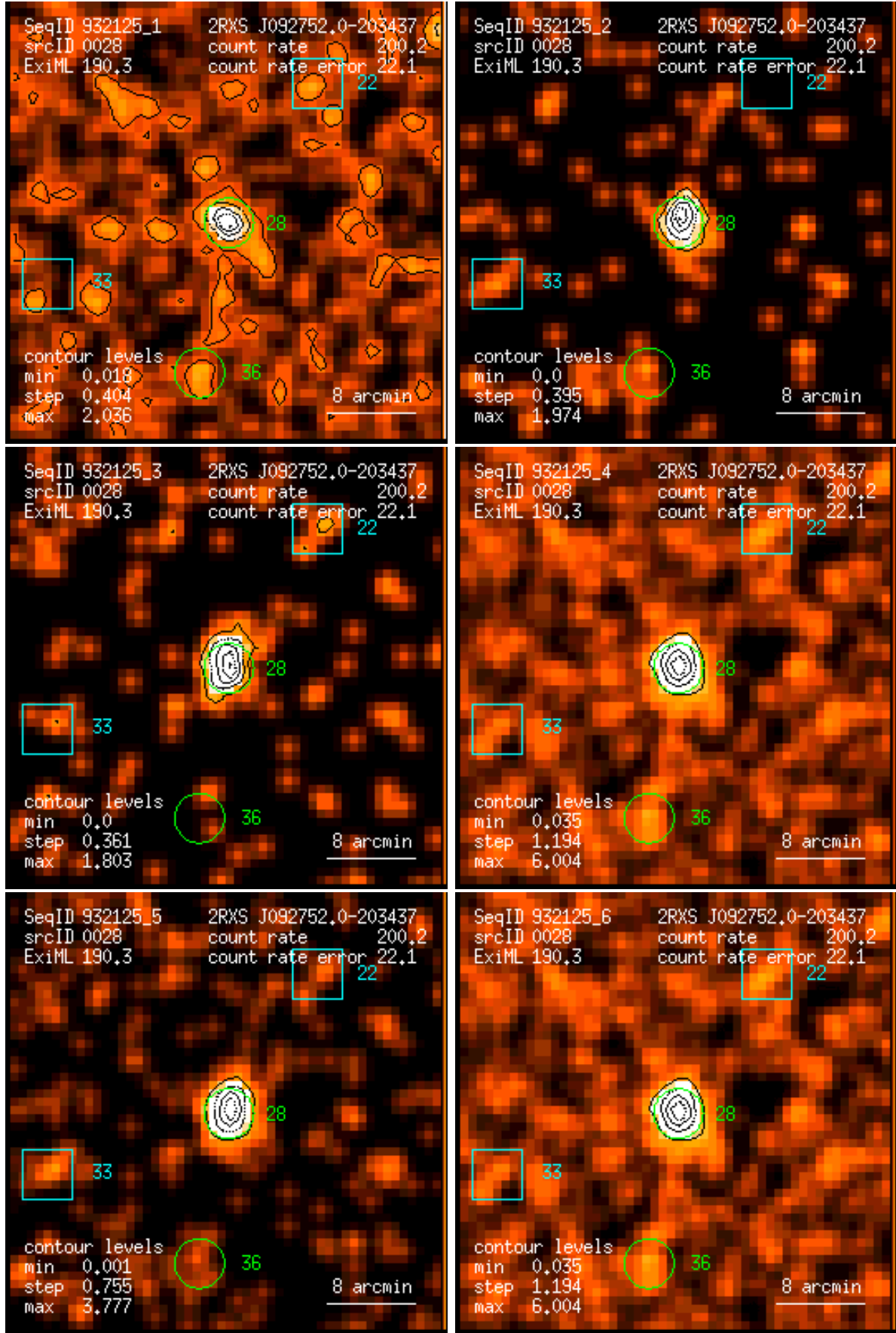
Figure 28: RASS 932125: detection 0028: band rate images, Gaussian filter: (1) PSPC channels 11 – 41, (2) 52 – 90, (3) 91 – 201, (4) 11 – 235, (5) 52 – 201, (6) 11 – 201. Broad band rates in counts/ks. Band rate contour levels in counts/ks/arcmin 2 .
