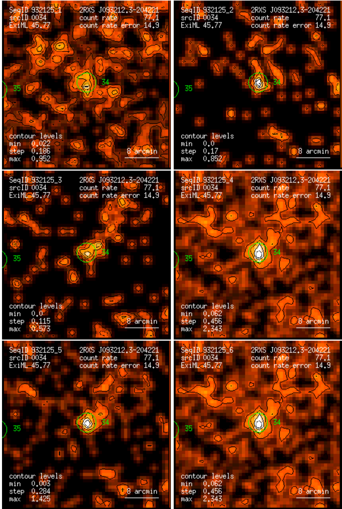
Figure 34: RASS 932125: detection 0034: band rate images, Gaussian filter: (1) PSPC channels 11 – 41, (2) 52 – 90, (3) 91 – 201, (4) 11 – 235, (5) 52 – 201, (6) 11 – 201. Broad band rates in counts/ks. Band rate contour levels in counts/ks/arcmin 2 .
