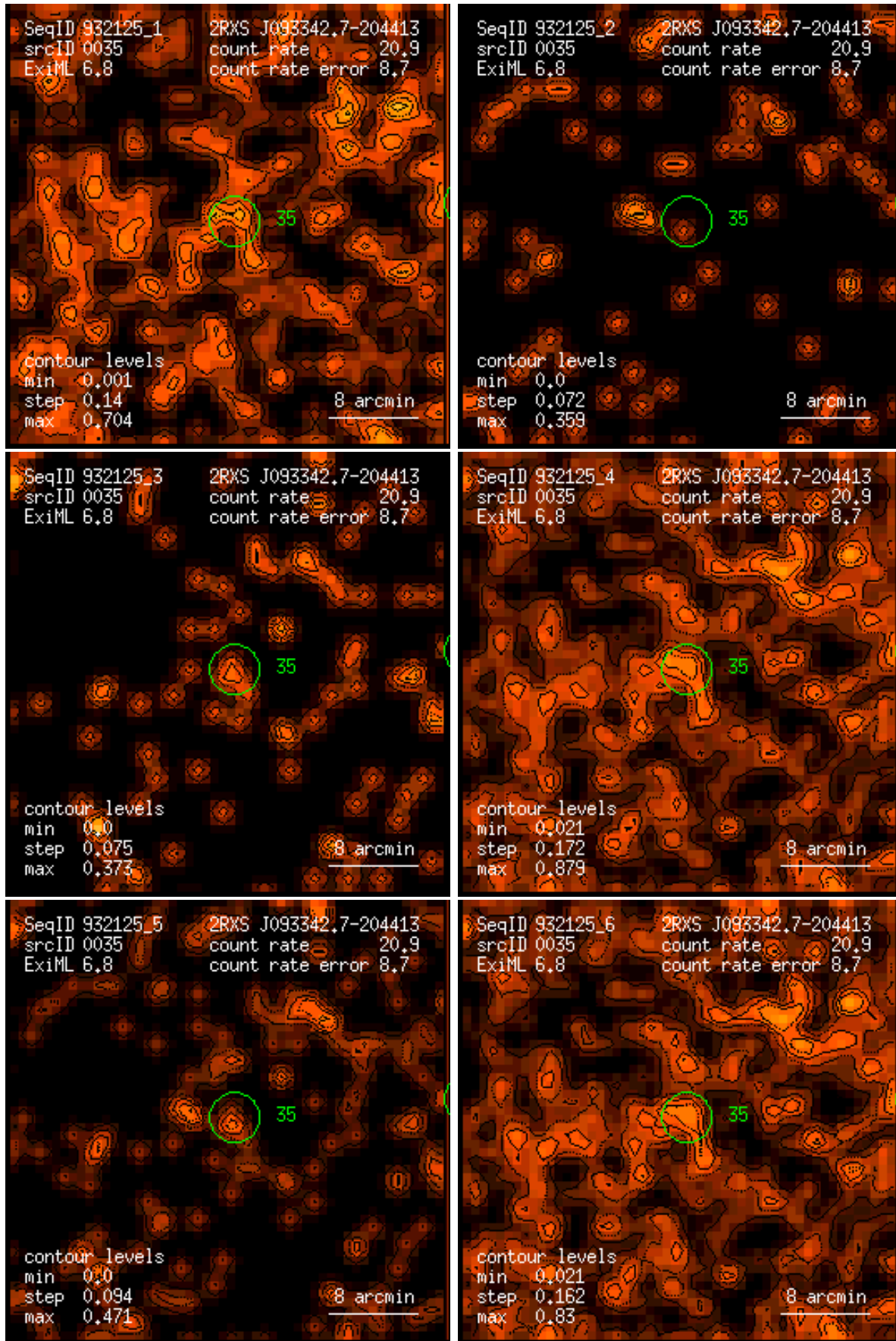
Figure 35: RASS 932125: detection 0035: band rate images, Gaussian filter: (1) PSPC channels 11 – 41, (2) 52 – 90, (3) 91 – 201, (4) 11 – 235, (5) 52 – 201, (6) 11 – 201. Broad band rates in counts/ks. Band rate contour levels in counts/ks/arcmin 2 .
