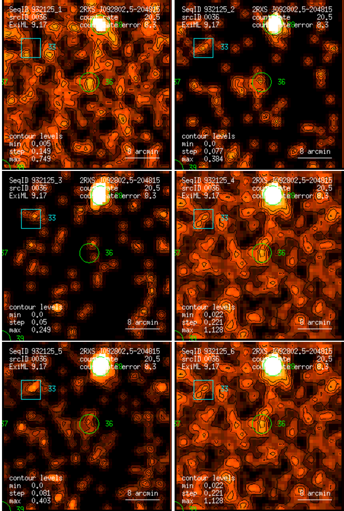
Figure 36: RASS 932125: detection 0036: band rate images, Gaussian filter: (1) PSPC channels 11 – 41, (2) 52 – 90, (3) 91 – 201, (4) 11 – 235, (5) 52 – 201, (6) 11 – 201. Broad band rates in counts/ks. Band rate contour levels in counts/ks/arcmin 2 .
