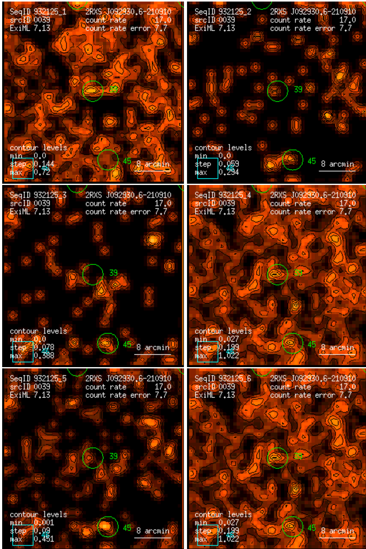
Figure 39: RASS 932125: detection 0039: band rate images, Gaussian filter: (1) PSPC channels 11 – 41, (2) 52 – 90, (3) 91 – 201, (4) 11 – 235, (5) 52 – 201, (6) 11 – 201. Broad band rates in counts/ks. Band rate contour levels in counts/ks/arcmin 2 .
