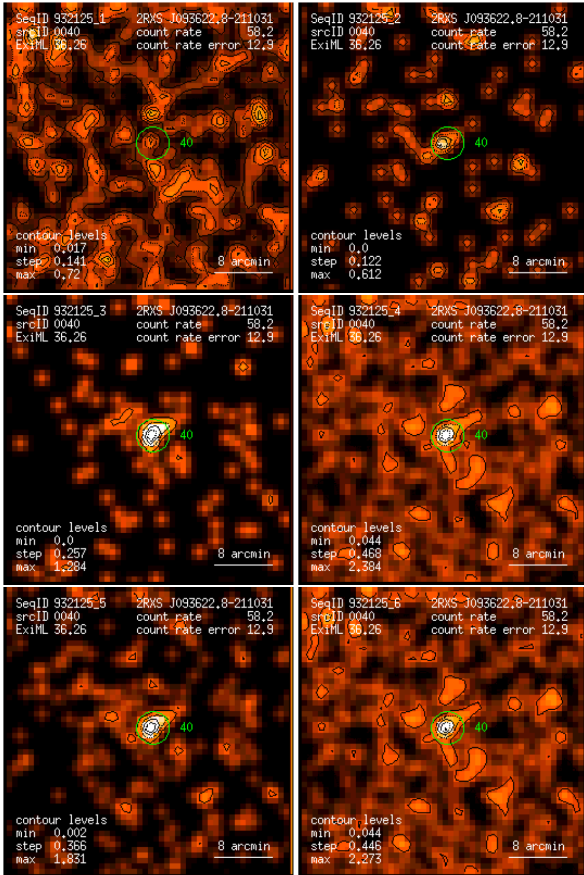
Figure 40: RASS 932125: detection 0040: band rate images, Gaussian filter: (1) PSPC channels 11 – 41, (2) 52 – 90, (3) 91 – 201, (4) 11 – 235, (5) 52 – 201, (6) 11 – 201. Broad band rates in counts/ks. Band rate contour levels in counts/ks/arcmin 2 .
