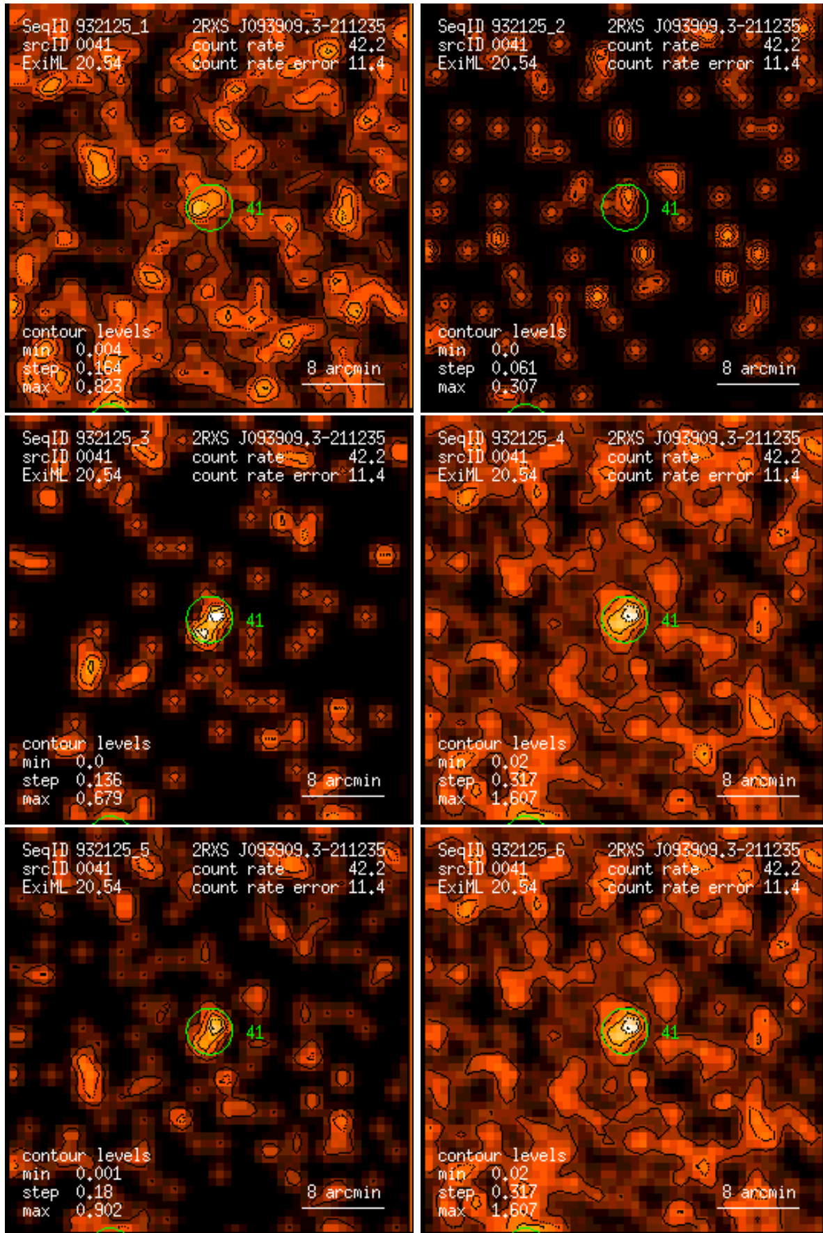
Figure 41: RASS 932125: detection 0041: band rate images, Gaussian filter: (1) PSPC channels 11 – 41, (2) 52 – 90, (3) 91 – 201, (4) 11 – 235, (5) 52 – 201, (6) 11 – 201. Broad band rates in counts/ks. Band rate contour levels in counts/ks/arcmin 2 .
