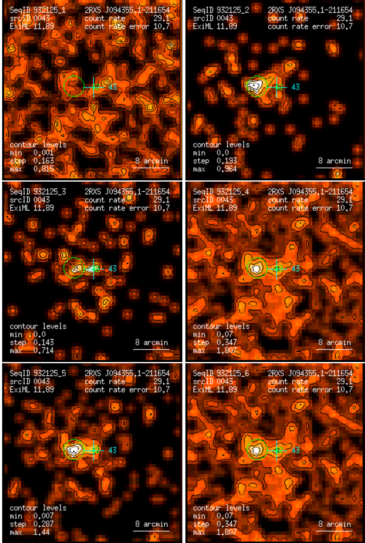
Figure 43: RASS 932125: detection 0043: band rate images, Gaussian filter: (1) PSPC channels 11 – 41, (2) 52 – 90, (3) 91 – 201, (4) 11 – 235, (5) 52 – 201, (6) 11 – 201. Broad band rates in counts/ks. Band rate contour levels in counts/ks/arcmin 2 .
