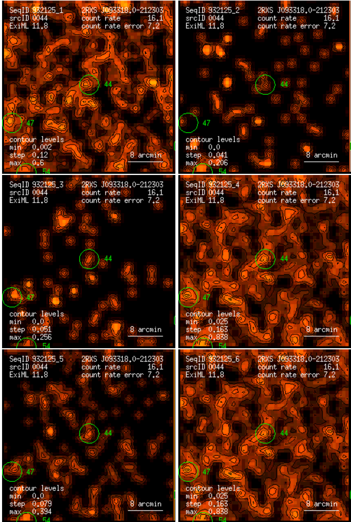
Figure 44: RASS 932125: detection 0044: band rate images, Gaussian filter: (1) PSPC channels 11 – 41, (2) 52 – 90, (3) 91 – 201, (4) 11 – 235, (5) 52 – 201, (6) 11 – 201. Broad band rates in counts/ks. Band rate contour levels in counts/ks/arcmin 2 .
