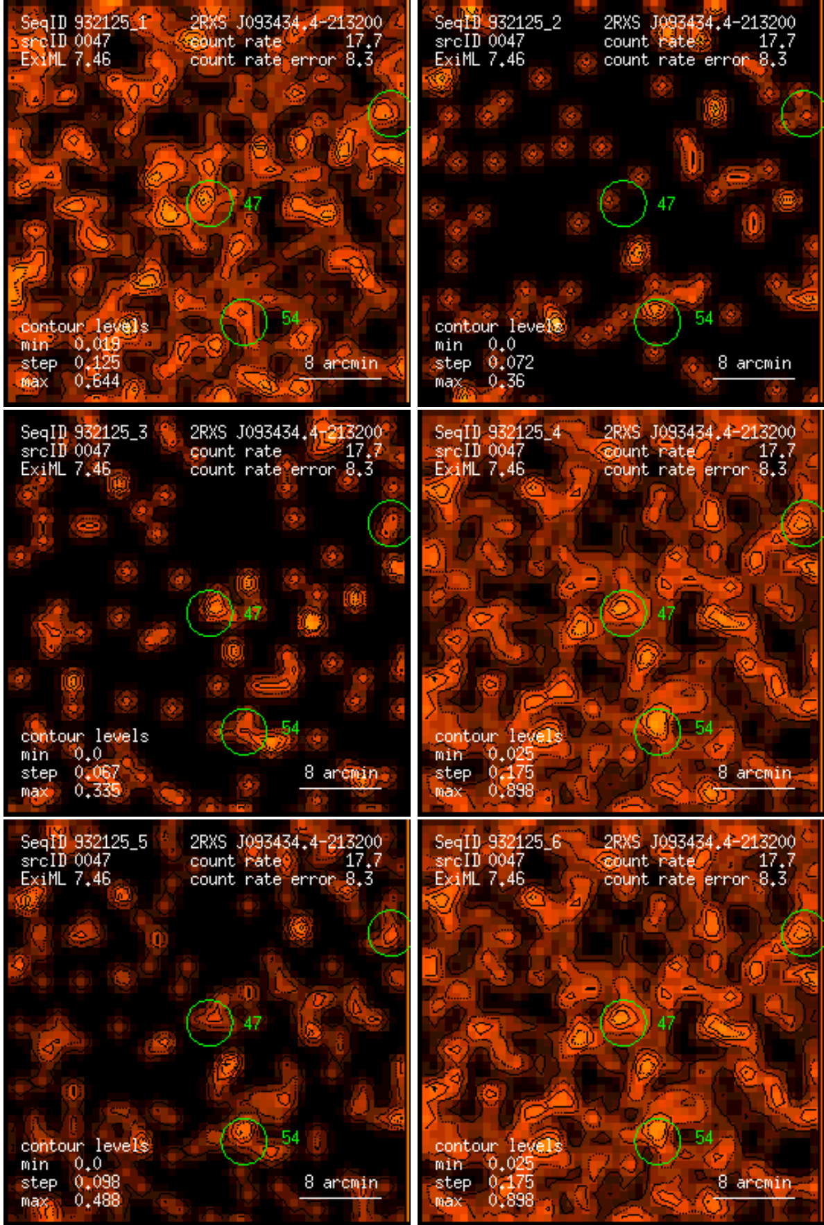
Figure 47: RASS 932125: detection 0047: band rate images, Gaussian filter: (1) PSPC channels 11 – 41, (2) 52 – 90, (3) 91 – 201, (4) 11 – 235, (5) 52 – 201, (6) 11 – 201. Broad band rates in counts/ks. Band rate contour levels in counts/ks/arcmin 2 .
