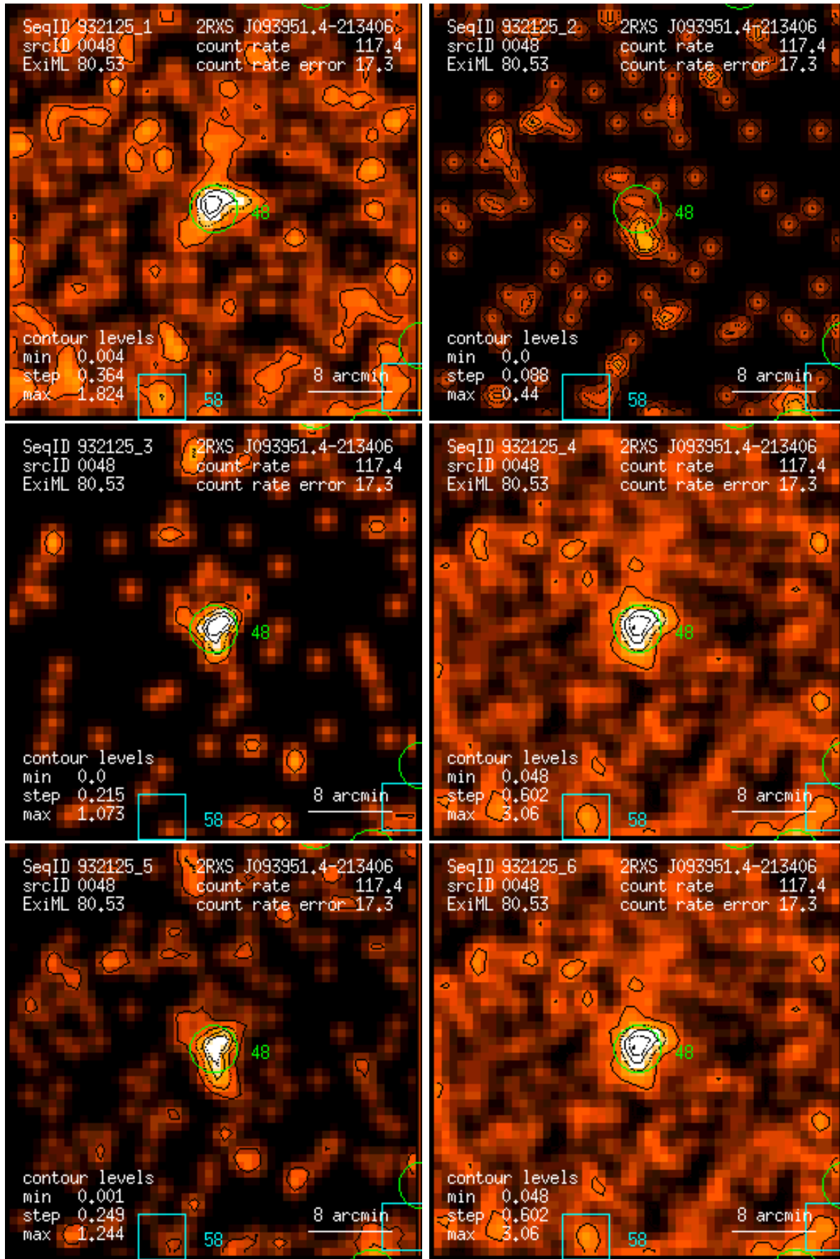
Figure 48: RASS 932125: detection 0048: band rate images, Gaussian filter: (1) PSPC channels 11 – 41, (2) 52 – 90, (3) 91 – 201, (4) 11 – 235, (5) 52 – 201, (6) 11 – 201. Broad band rates in counts/ks. Band rate contour levels in counts/ks/arcmin 2 .
