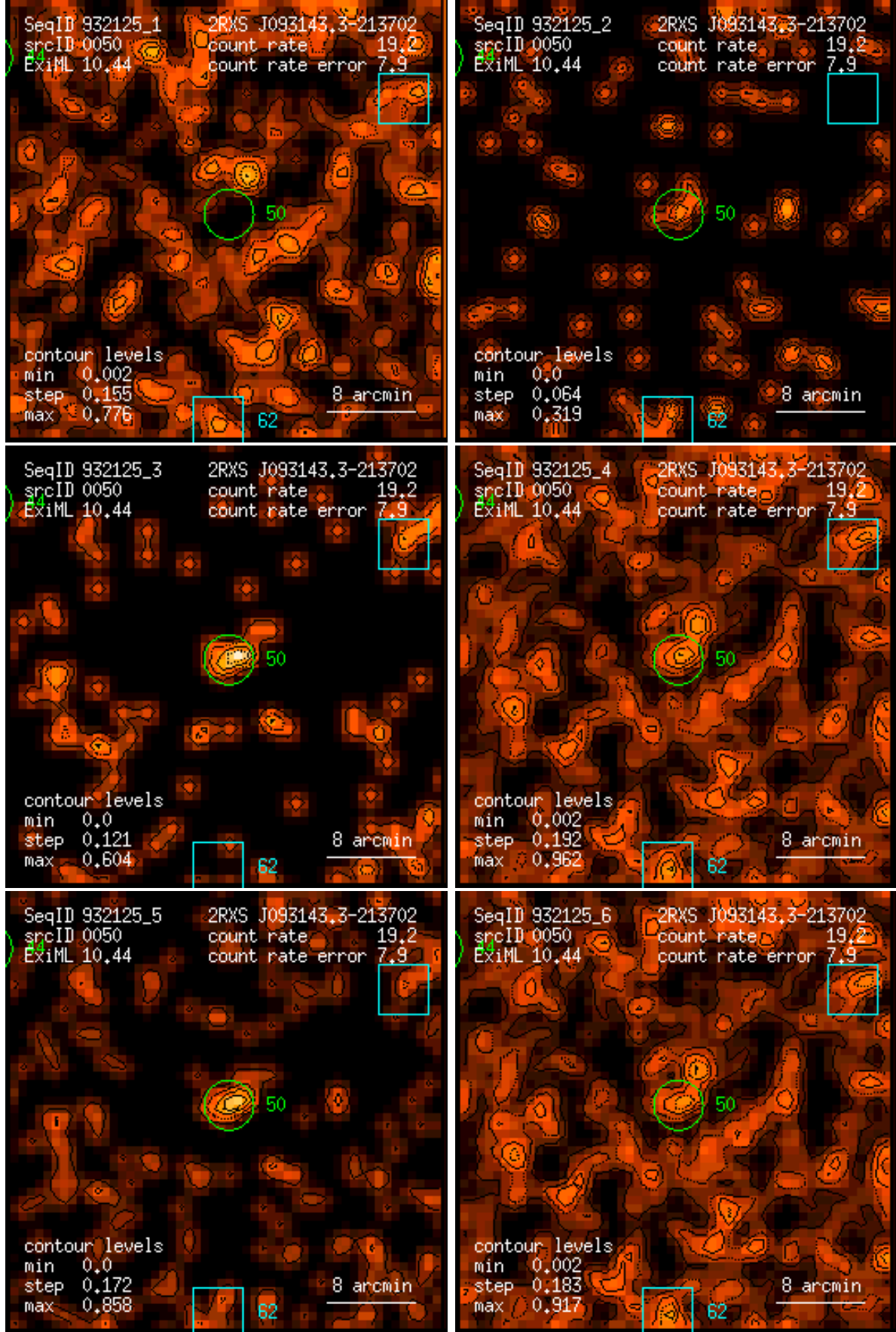
Figure 50: RASS 932125: detection 0050: band rate images, Gaussian filter: (1) PSPC channels 11 – 41, (2) 52 – 90, (3) 91 – 201, (4) 11 – 235, (5) 52 – 201, (6) 11 – 201. Broad band rates in counts/ks. Band rate contour levels in counts/ks/arcmin 2 .
