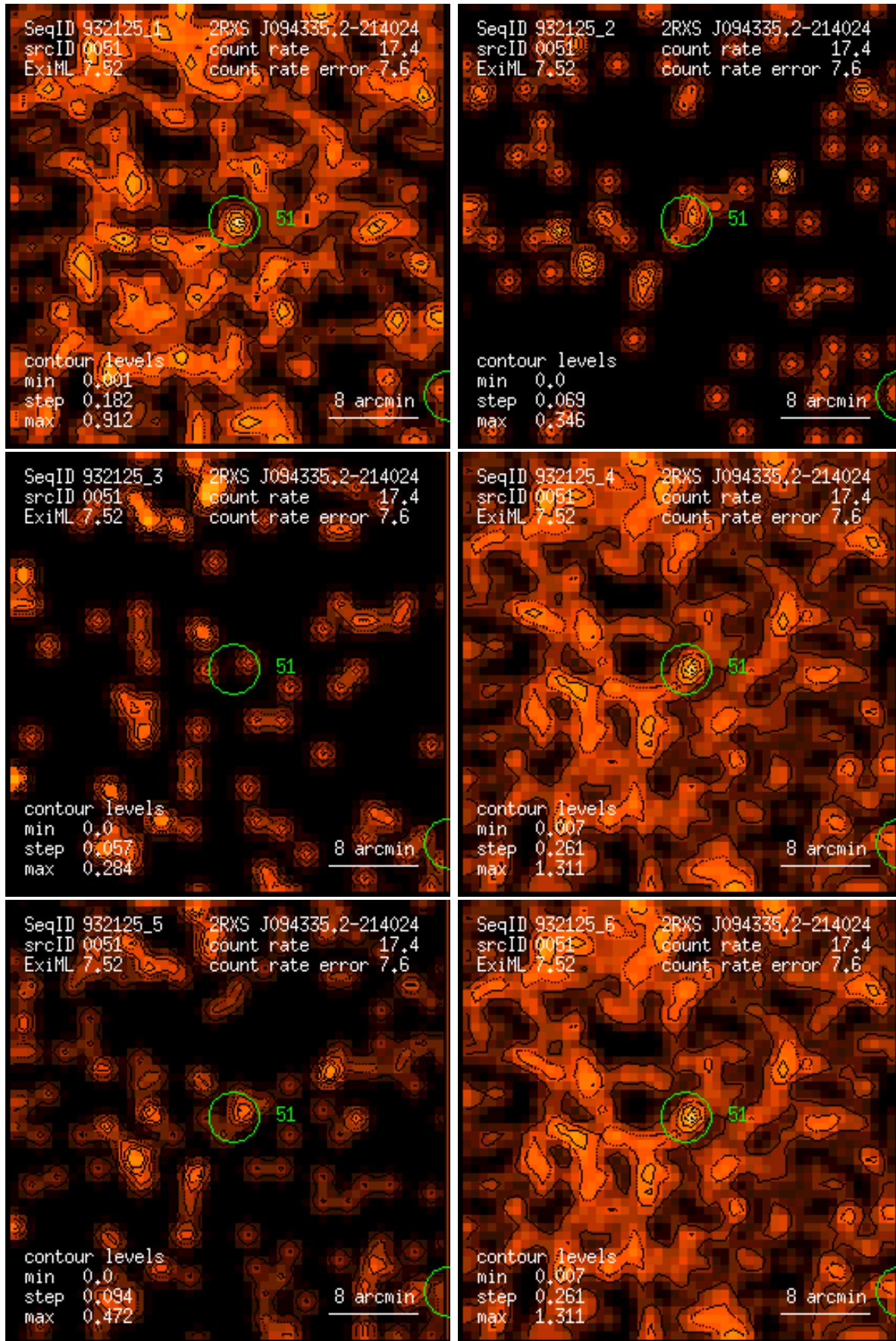
Figure 51: RASS 932125: detection 0051: band rate images, Gaussian filter: (1) PSPC channels 11 – 41, (2) 52 – 90, (3) 91 – 201, (4) 11 – 235, (5) 52 – 201, (6) 11 – 201. Broad band rates in counts/ks. Band rate contour levels in counts/ks/arcmin 2 .
