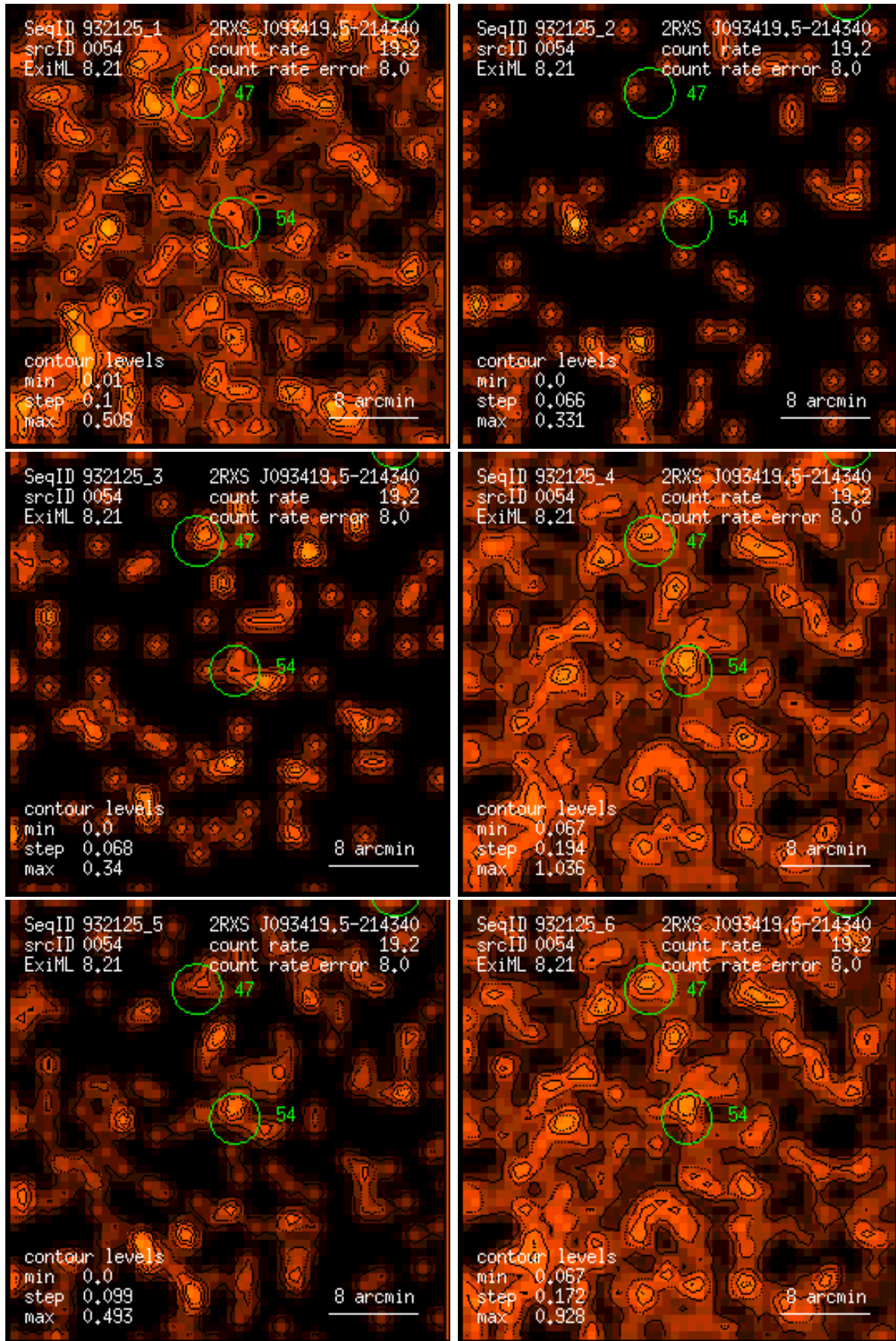
Figure 54: RASS 932125: detection 0054: band rate images, Gaussian filter: (1) PSPC channels 11 – 41, (2) 52 – 90, (3) 91 – 201, (4) 11 – 235, (5) 52 – 201, (6) 11 – 201. Broad band rates in counts/ks. Band rate contour levels in counts/ks/arcmin 2 .
