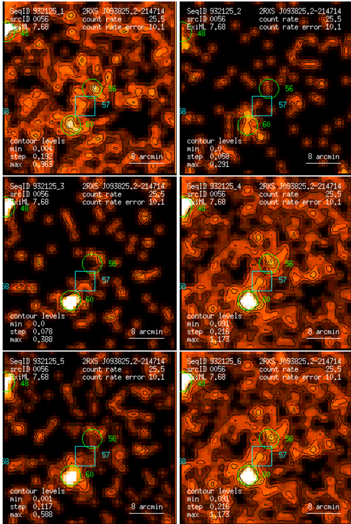
Figure 56: RASS 932125: detection 0056: band rate images, Gaussian filter: (1) PSPC channels 11 – 41, (2) 52 – 90, (3) 91 – 201, (4) 11 – 235, (5) 52 – 201, (6) 11 – 201. Broad band rates in counts/ks. Band rate contour levels in counts/ks/arcmin 2 .
