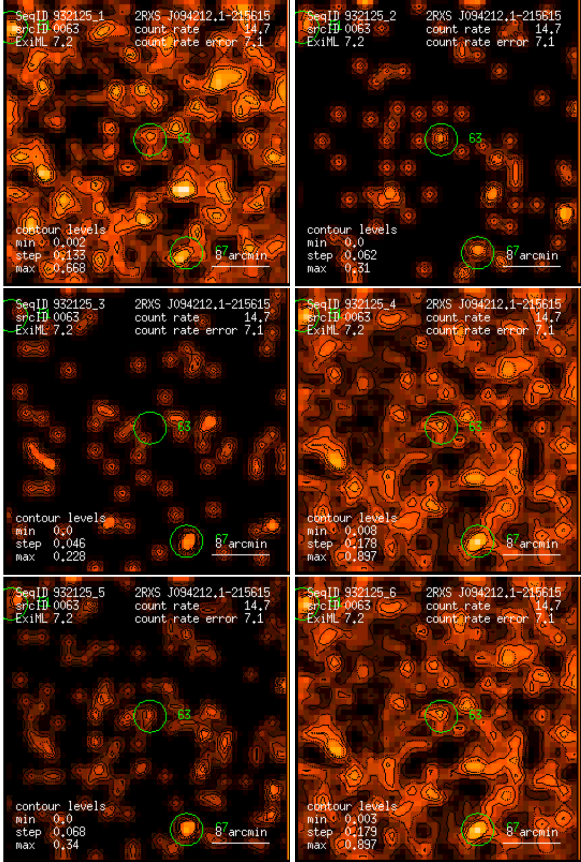
Figure 63: RASS 932125: detection 0063: band rate images, Gaussian filter: (1) PSPC channels 11 – 41, (2) 52 – 90, (3) 91 – 201, (4) 11 – 235, (5) 52 – 201, (6) 11 – 201. Broad band rates in counts/ks. Band rate contour levels in counts/ks/arcmin 2 .
