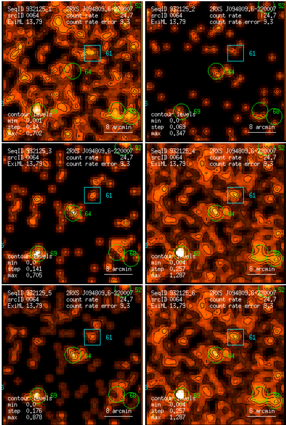
Figure 64: RASS 932125: detection 0064: band rate images, Gaussian filter: (1) PSPC channels 11 – 41, (2) 52 – 90, (3) 91 – 201, (4) 11 – 235, (5) 52 – 201, (6) 11 – 201. Broad band rates in counts/ks. Band rate contour levels in counts/ks/arcmin 2 .
