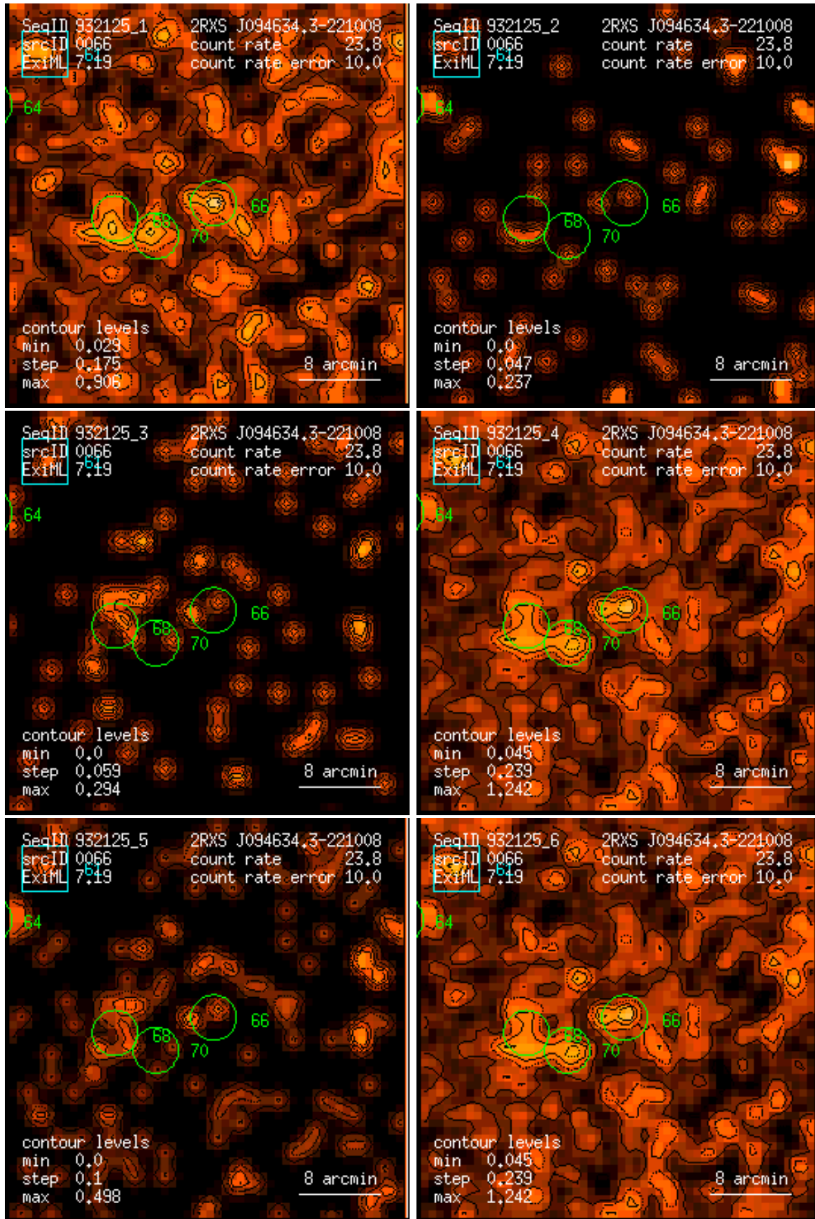
Figure 66: RASS 932125: detection 0066: band rate images, Gaussian filter: (1) PSPC channels 11 – 41, (2) 52 – 90, (3) 91 – 201, (4) 11 – 235, (5) 52 – 201, (6) 11 – 201. Broad band rates in counts/ks. Band rate contour levels in counts/ks/arcmin 2 .
