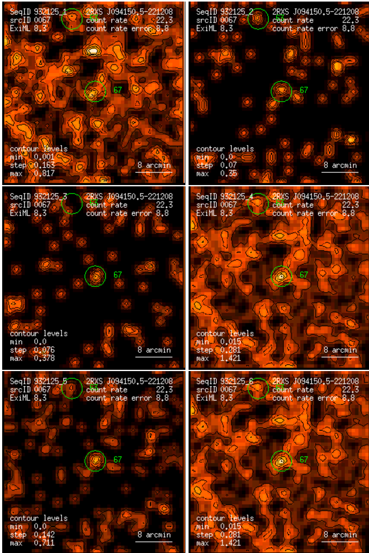
Figure 67: RASS 932125: detection 0067: band rate images, Gaussian filter: (1) PSPC channels 11 – 41, (2) 52 – 90, (3) 91 – 201, (4) 11 – 235, (5) 52 – 201, (6) 11 – 201. Broad band rates in counts/ks. Band rate contour levels in counts/ks/arcmin 2 .
