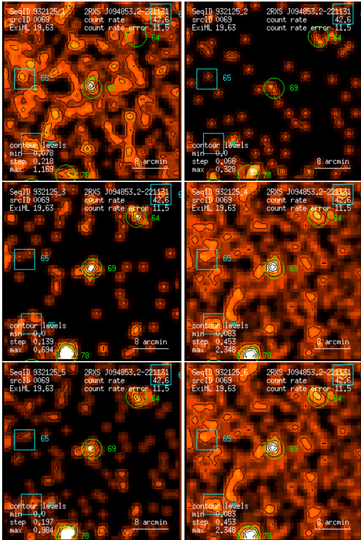
Figure 69: RASS 932125: detection 0069: band rate images, Gaussian filter: (1) PSPC channels 11 – 41, (2) 52 – 90, (3) 91 – 201, (4) 11 – 235, (5) 52 – 201, (6) 11 – 201. Broad band rates in counts/ks. Band rate contour levels in counts/ks/arcmin 2 .
