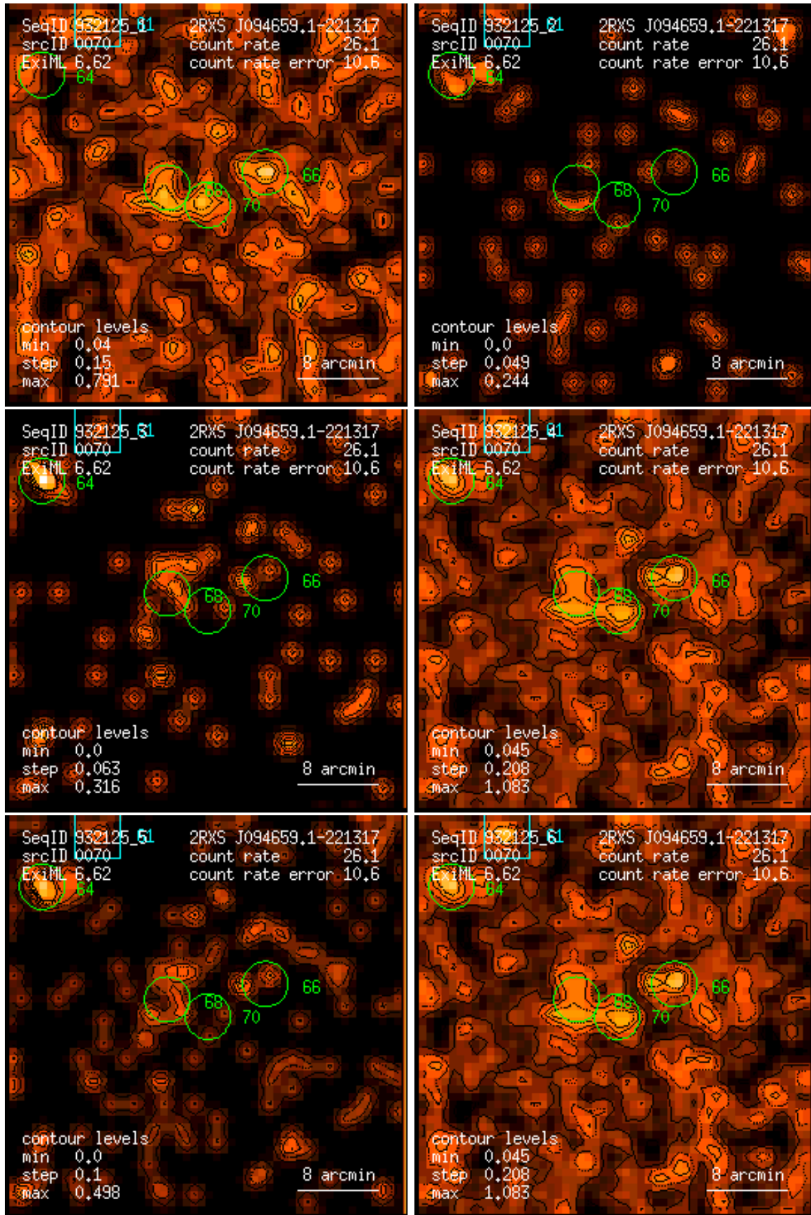
Figure 70: RASS 932125: detection 0070: band rate images, Gaussian filter: (1) PSPC channels 11 – 41, (2) 52 – 90, (3) 91 – 201, (4) 11 – 235, (5) 52 – 201, (6) 11 – 201. Broad band rates in counts/ks. Band rate contour levels in counts/ks/arcmin 2 .
