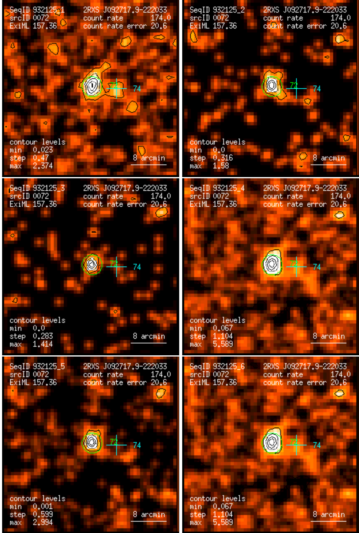
Figure 72: RASS 932125: detection 0072: band rate images, Gaussian filter: (1) PSPC channels 11 – 41, (2) 52 – 90, (3) 91 – 201, (4) 11 – 235, (5) 52 – 201, (6) 11 – 201. Broad band rates in counts/ks. Band rate contour levels in counts/ks/arcmin 2 .
