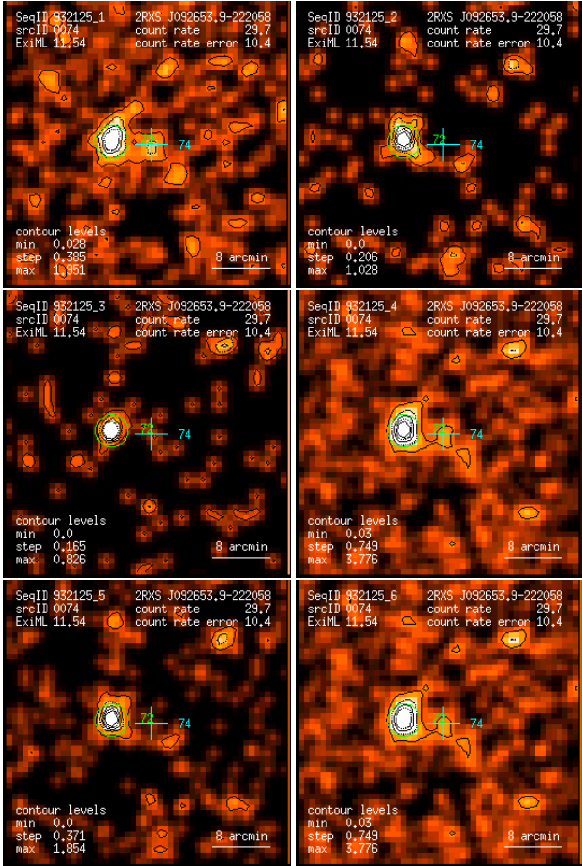
Figure 74: RASS 932125: detection 0074: band rate images, Gaussian filter: (1) PSPC channels 11 – 41, (2) 52 – 90, (3) 91 – 201, (4) 11 – 235, (5) 52 – 201, (6) 11 – 201. Broad band rates in counts/ks. Band rate contour levels in counts/ks/arcmin 2 .
