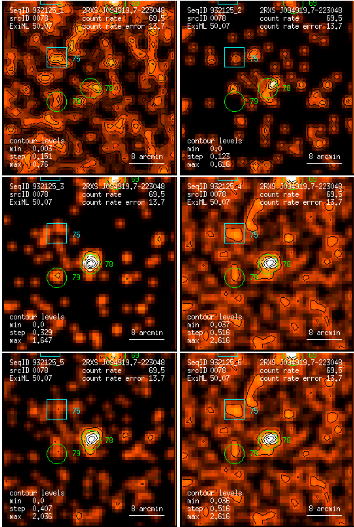
Figure 78: RASS 932125: detection 0078: band rate images, Gaussian filter: (1) PSPC channels 11 – 41, (2) 52 – 90, (3) 91 – 201, (4) 11 – 235, (5) 52 – 201, (6) 11 – 201. Broad band rates in counts/ks. Band rate contour levels in counts/ks/arcmin 2 .
