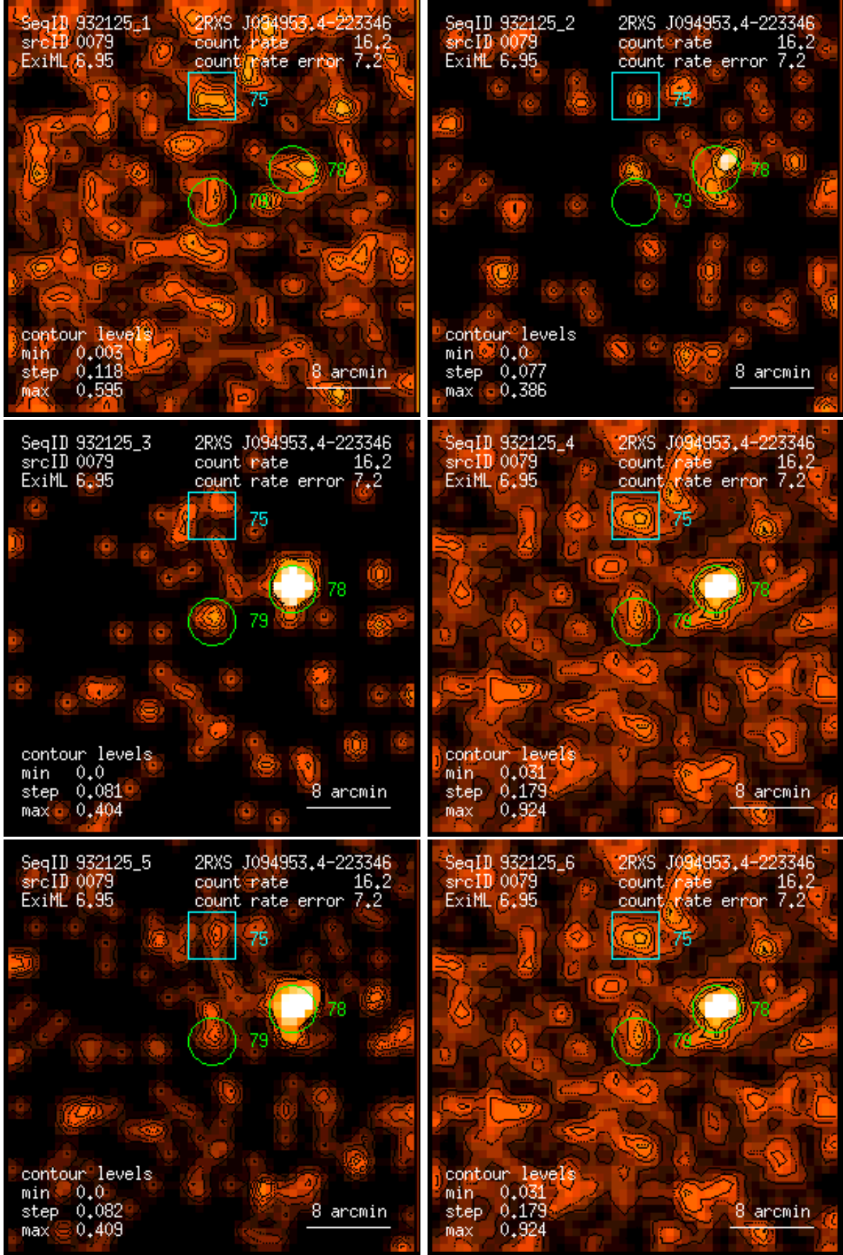
Figure 79: RASS 932125: detection 0079: band rate images, Gaussian filter: (1) PSPC channels 11 – 41, (2) 52 – 90, (3) 91 – 201, (4) 11 – 235, (5) 52 – 201, (6) 11 – 201. Broad band rates in counts/ks. Band rate contour levels in counts/ks/arcmin 2 .
