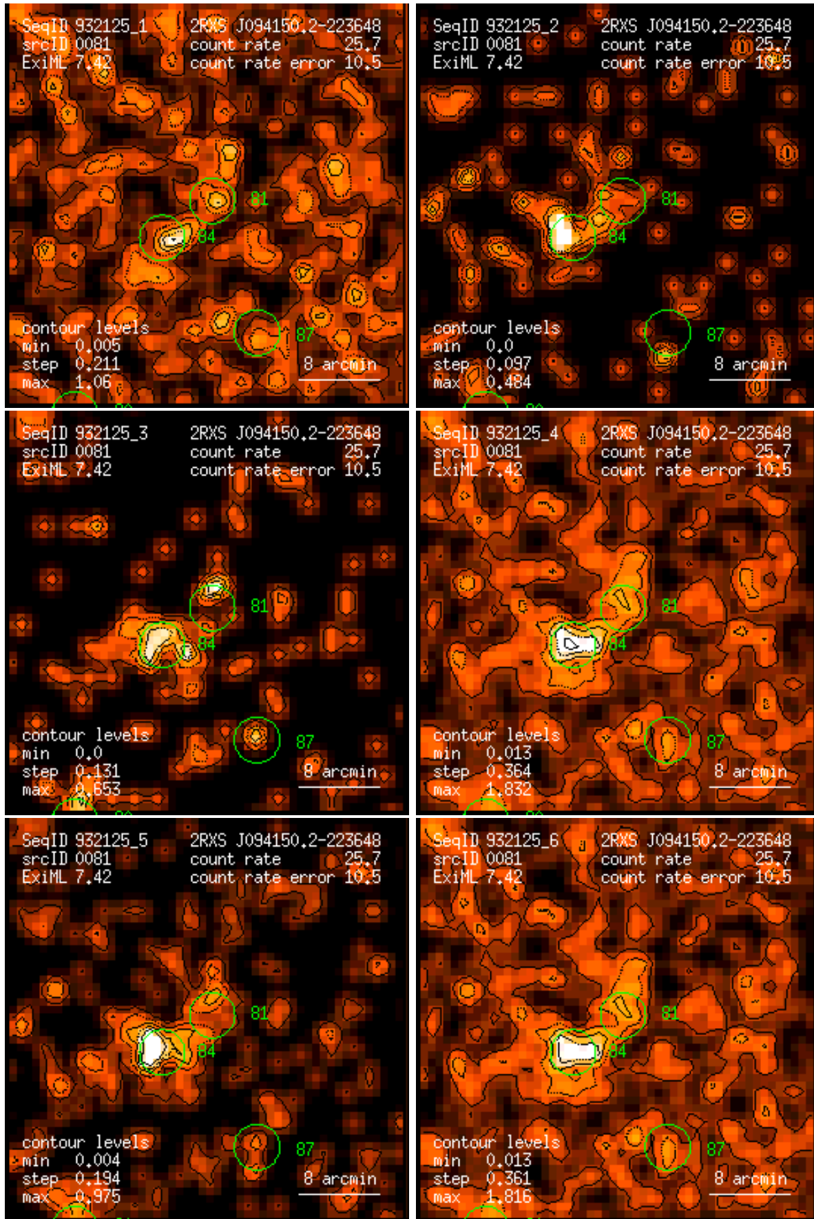
Figure 81: RASS 932125: detection 0081: band rate images, Gaussian filter: (1) PSPC channels 11 – 41, (2) 52 – 90, (3) 91 – 201, (4) 11 – 235, (5) 52 – 201, (6) 11 – 201. Broad band rates in counts/ks. Band rate contour levels in counts/ks/arcmin 2 .
