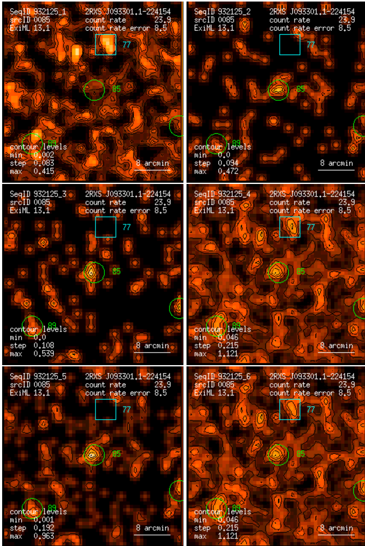
Figure 85: RASS 932125: detection 0085: band rate images, Gaussian filter: (1) PSPC channels 11 – 41, (2) 52 – 90, (3) 91 – 201, (4) 11 – 235, (5) 52 – 201, (6) 11 – 201. Broad band rates in counts/ks. Band rate contour levels in counts/ks/arcmin 2 .
