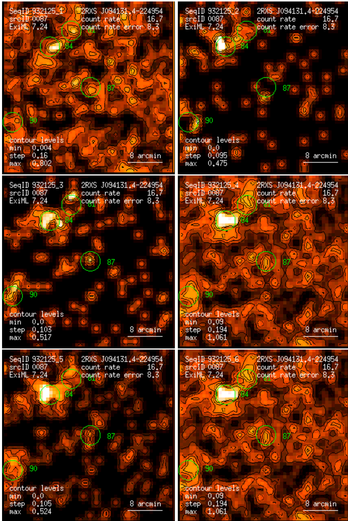
Figure 87: RASS 932125: detection 0087: band rate images, Gaussian filter: (1) PSPC channels 11 – 41, (2) 52 – 90, (3) 91 – 201, (4) 11 – 235, (5) 52 – 201, (6) 11 – 201. Broad band rates in counts/ks. Band rate contour levels in counts/ks/arcmin 2 .
