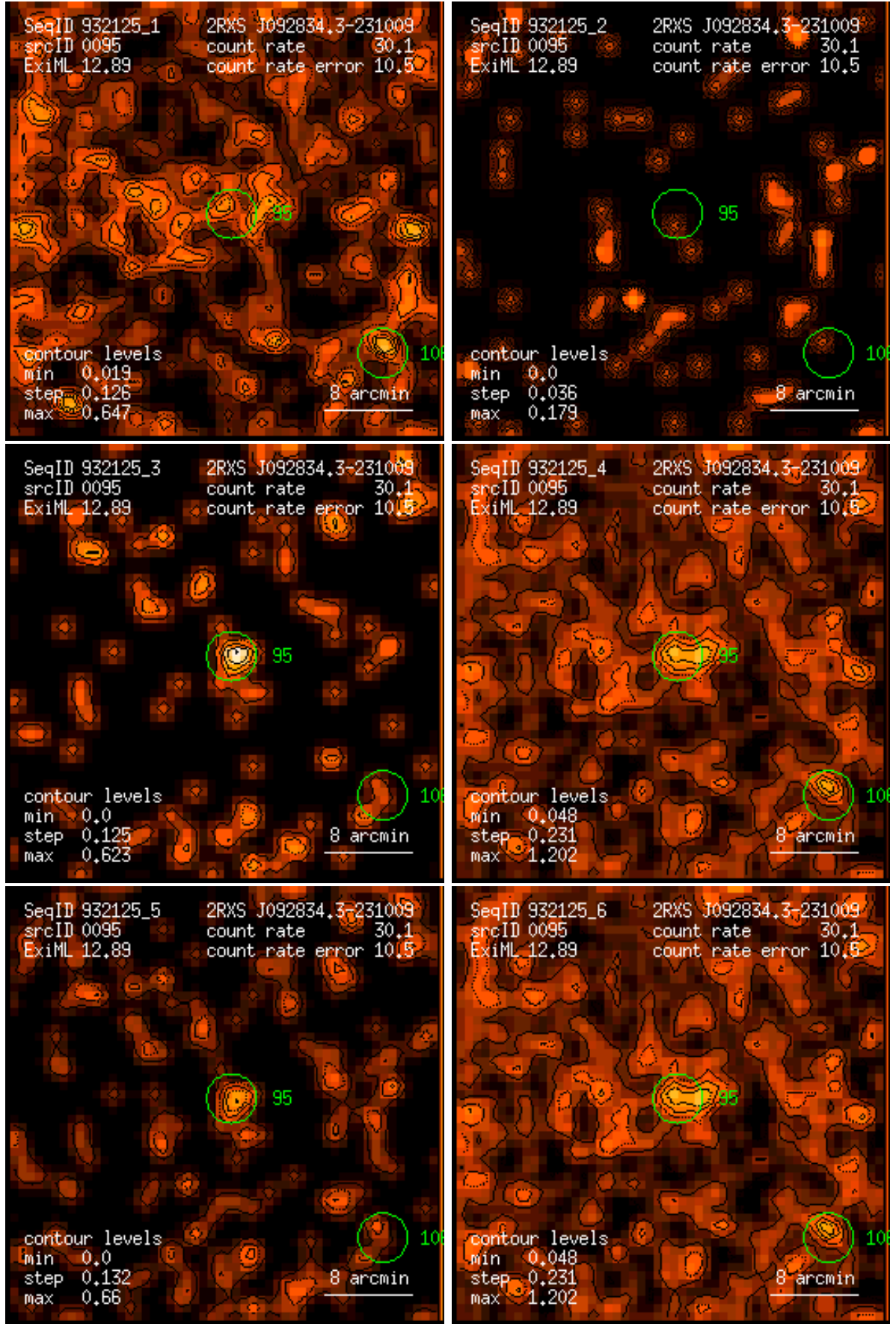
Figure 95: RASS 932125: detection 0095: band rate images, Gaussian filter: (1) PSPC channels 11 – 41, (2) 52 – 90, (3) 91 – 201, (4) 11 – 235, (5) 52 – 201, (6) 11 – 201. Broad band rates in counts/ks. Band rate contour levels in counts/ks/arcmin 2 .
