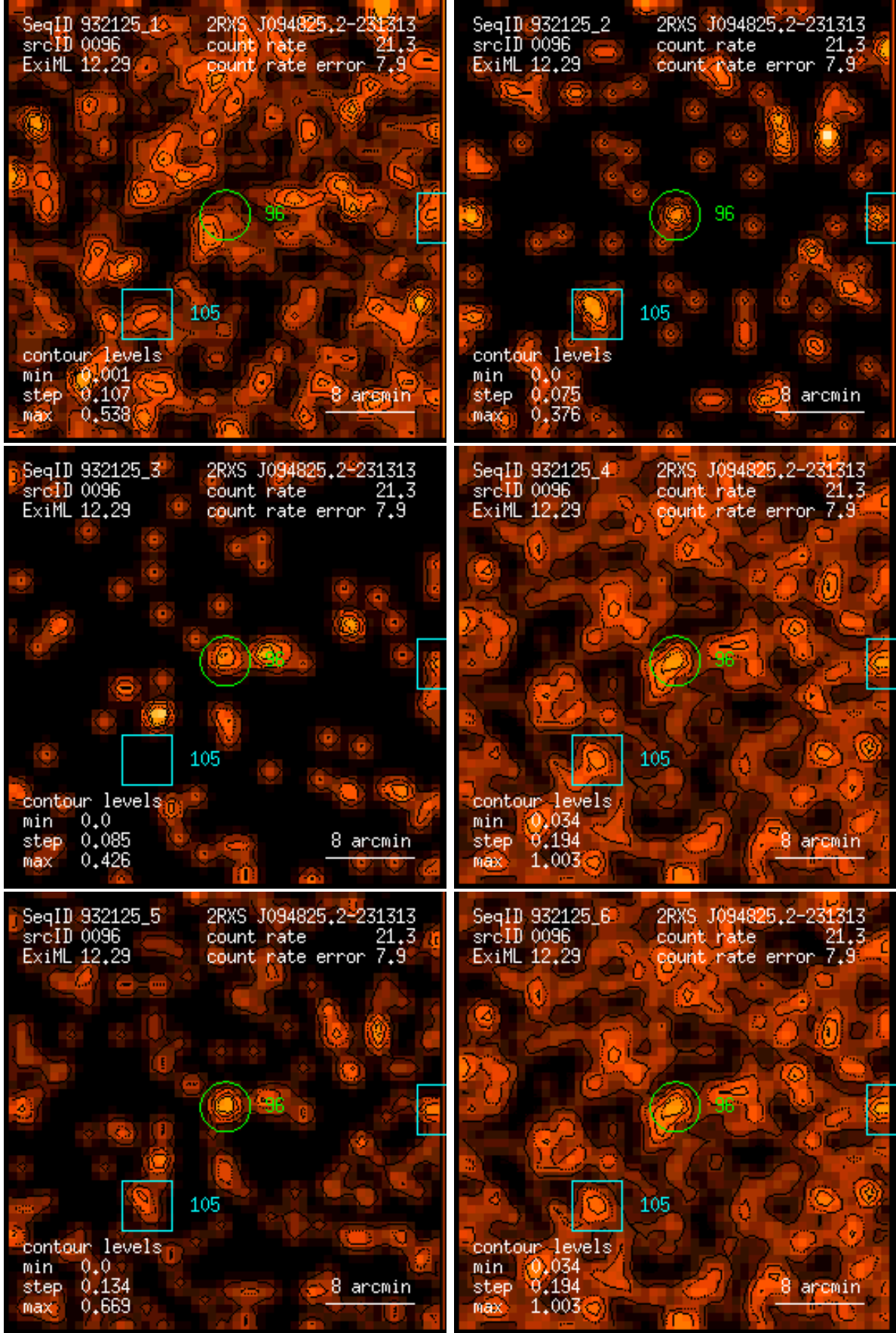
Figure 96: RASS 932125: detection 0096: band rate images, Gaussian filter: (1) PSPC channels 11 – 41, (2) 52 – 90, (3) 91 – 201, (4) 11 – 235, (5) 52 – 201, (6) 11 – 201. Broad band rates in counts/ks. Band rate contour levels in counts/ks/arcmin 2 .
