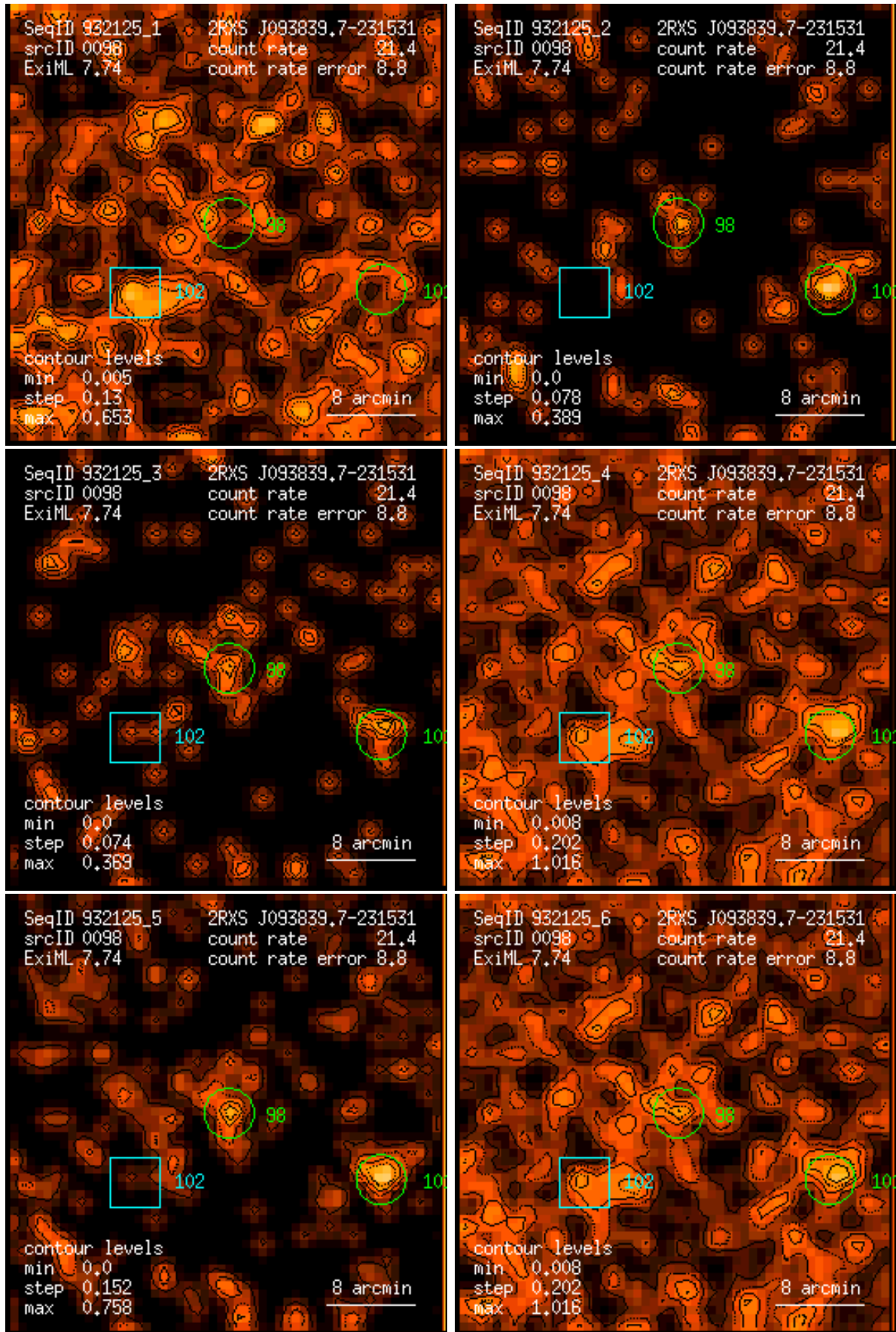
Figure 98: RASS 932125: detection 0098: band rate images, Gaussian filter: (1) PSPC channels 11 – 41, (2) 52 – 90, (3) 91 – 201, (4) 11 – 235, (5) 52 – 201, (6) 11 – 201. Broad band rates in counts/ks. Band rate contour levels in counts/ks/arcmin 2 .
