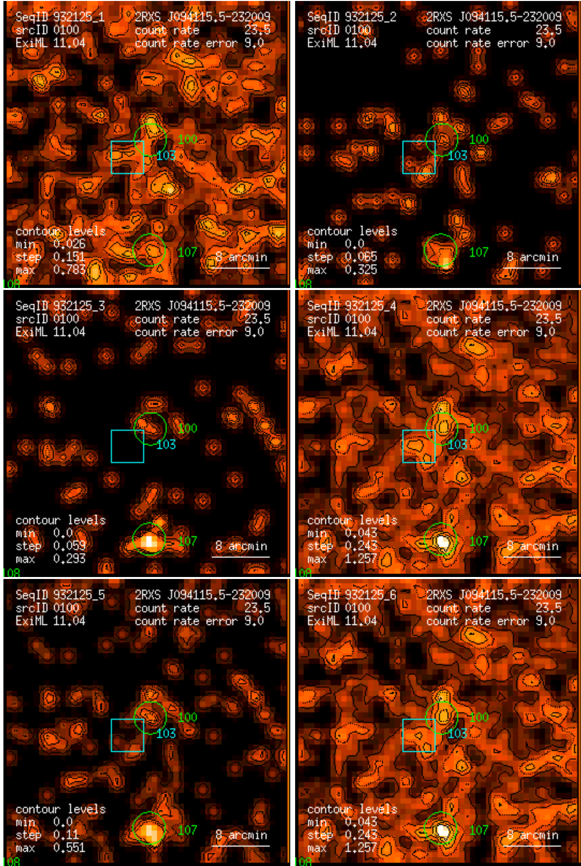
Figure 100: RASS 932125: detection 0100: band rate images, Gaussian filter: (1) PSPC channels 11 – 41, (2) 52 – 90, (3) 91 – 201, (4) 11 – 235, (5) 52 – 201, (6) 11 – 201. Broad band rates in counts/ks. Band rate contour levels in counts/ks/arcmin 2 .
