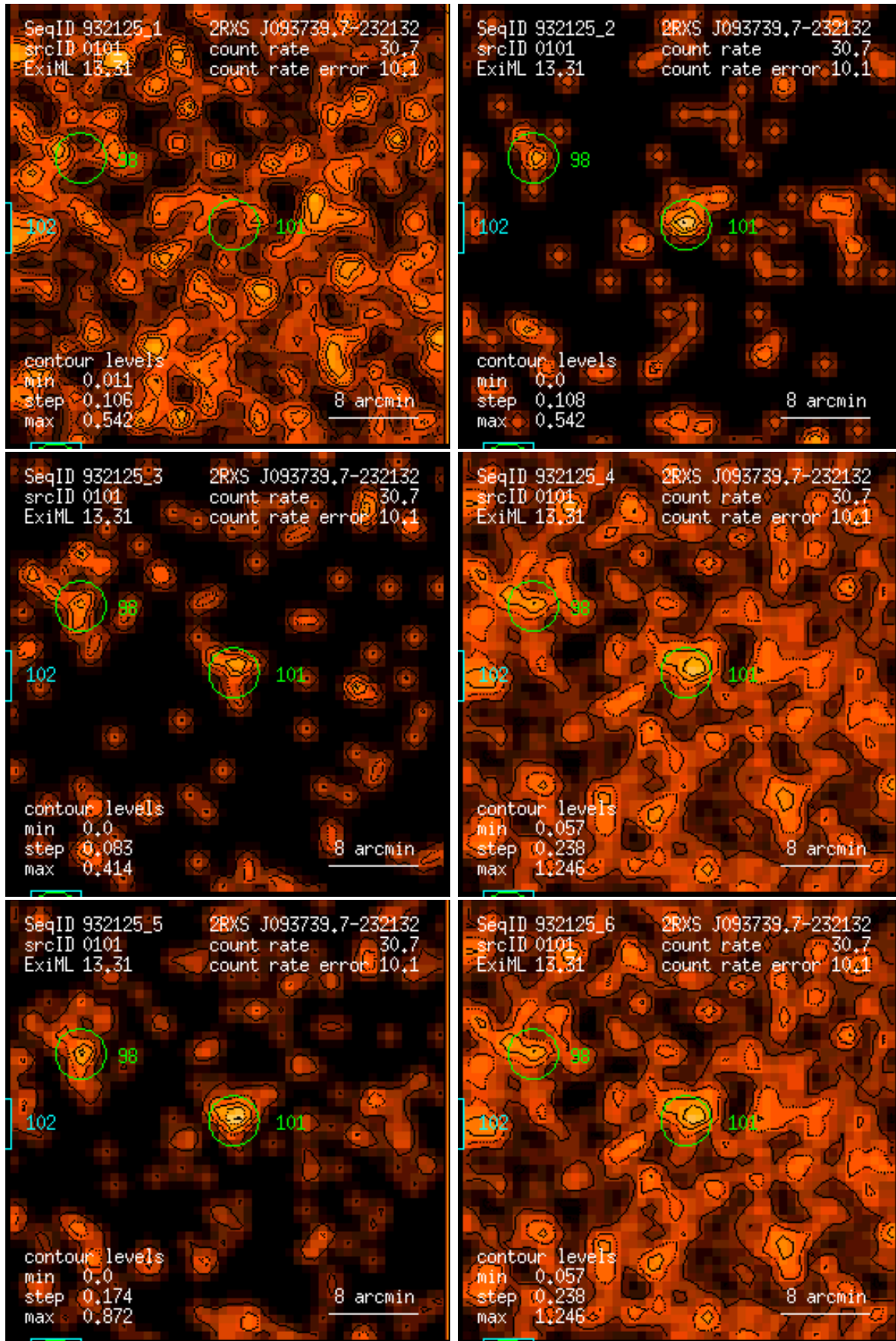
Figure 101: RASS 932125: detection 0101: band rate images, Gaussian filter: (1) PSPC channels 11 – 41, (2) 52 – 90, (3) 91 – 201, (4) 11 – 235, (5) 52 – 201, (6) 11 – 201. Broad band rates in counts/ks. Band rate contour levels in counts/ks/arcmin 2 .
