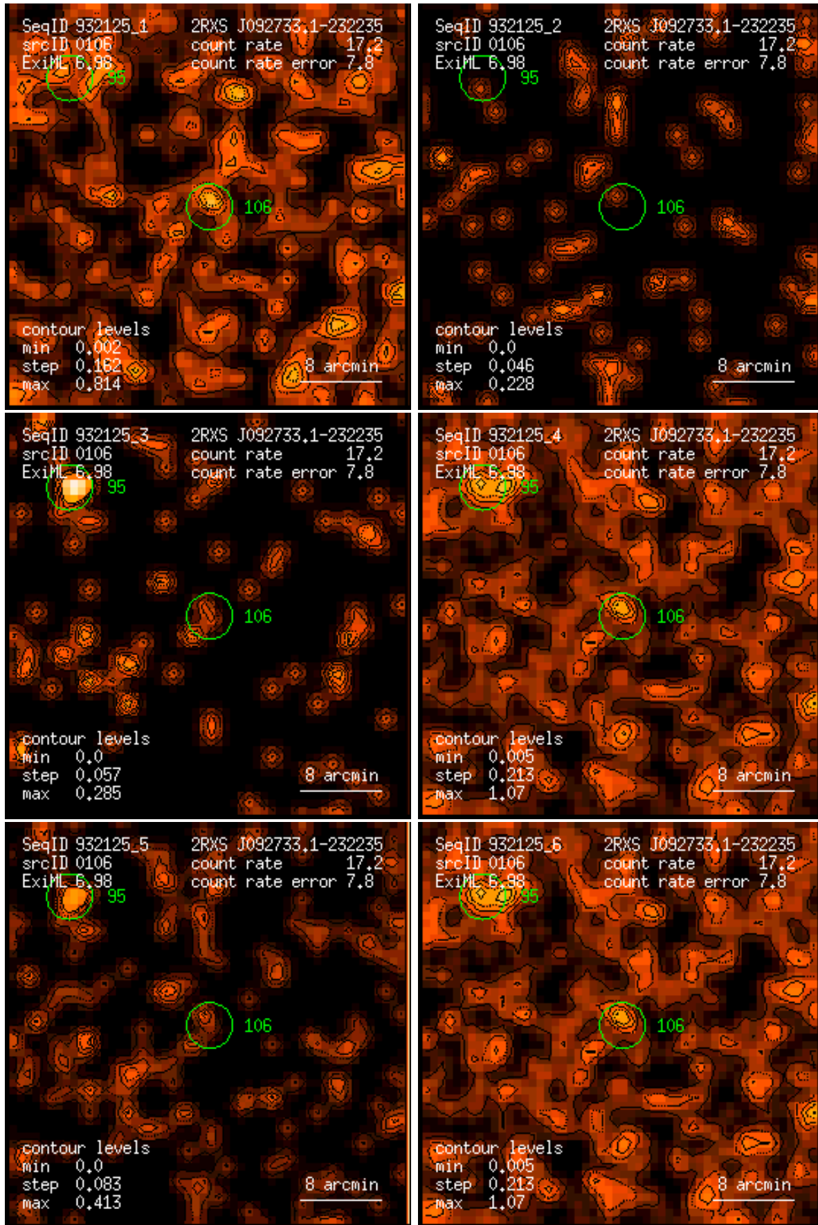
Figure 106: RASS 932125: detection 0106: band rate images, Gaussian filter: (1) PSPC channels 11 – 41, (2) 52 – 90, (3) 91 – 201, (4) 11 – 235, (5) 52 – 201, (6) 11 – 201. Broad band rates in counts/ks. Band rate contour levels in counts/ks/arcmin 2 .
