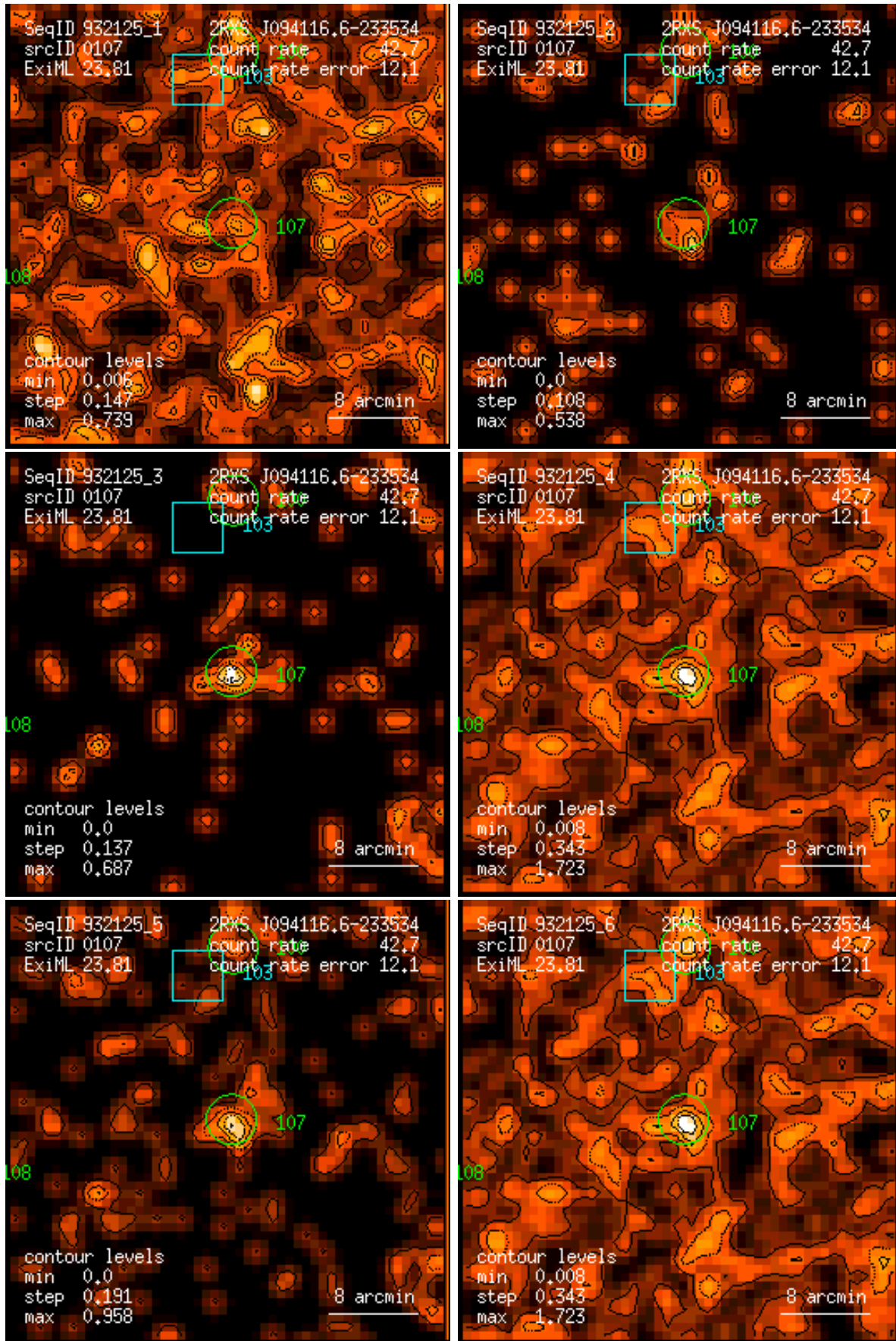
Figure 107: RASS 932125: detection 0107: band rate images, Gaussian filter: (1) PSPC channels 11 – 41, (2) 52 – 90, (3) 91 – 201, (4) 11 – 235, (5) 52 – 201, (6) 11 – 201. Broad band rates in counts/ks. Band rate contour levels in counts/ks/arcmin 2 .
