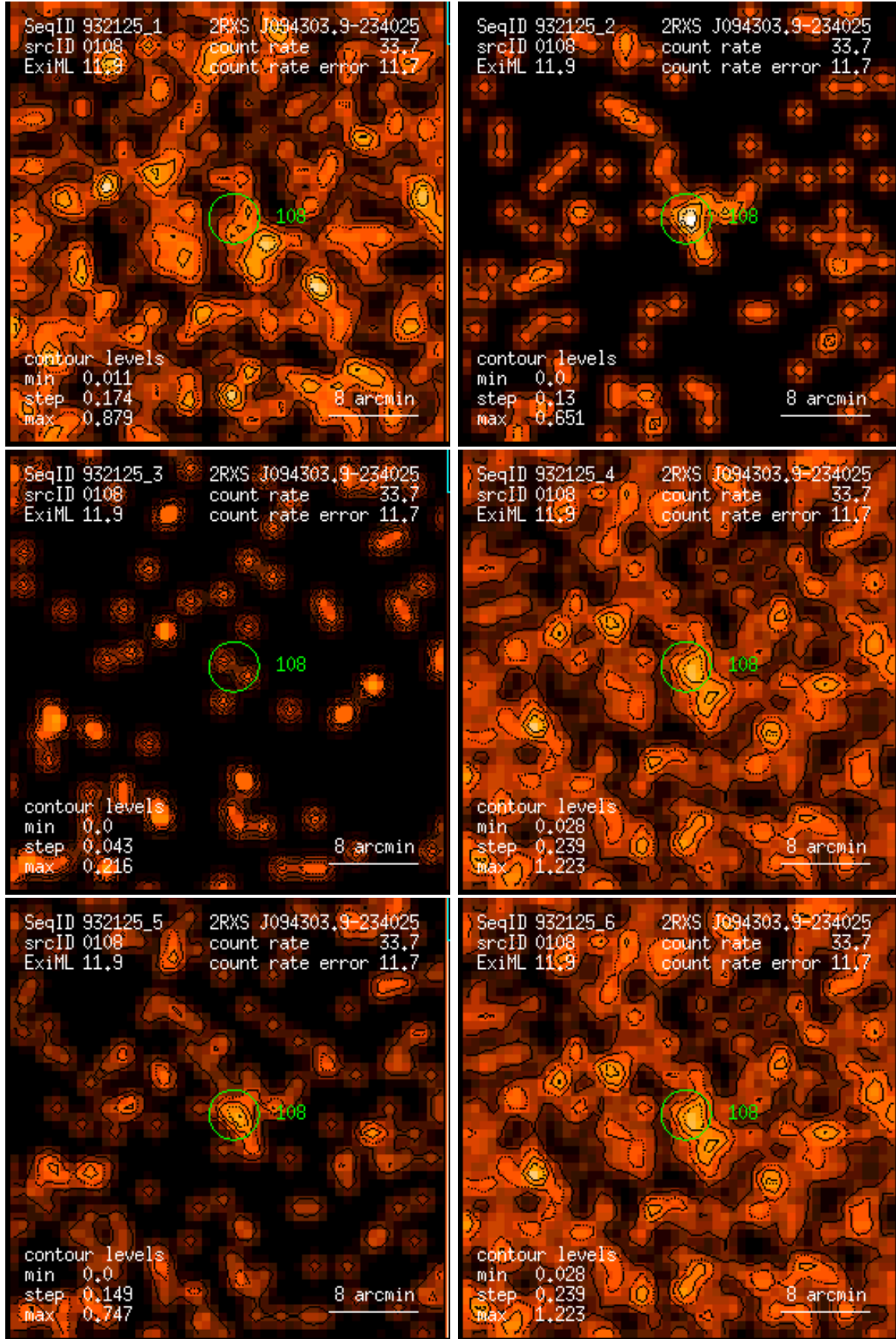
Figure 108: RASS 932125: detection 0108: band rate images, Gaussian filter: (1) PSPC channels 11 – 41, (2) 52 – 90, (3) 91 – 201, (4) 11 – 235, (5) 52 – 201, (6) 11 – 201. Broad band rates in counts/ks. Band rate contour levels in counts/ks/arcmin 2 .
