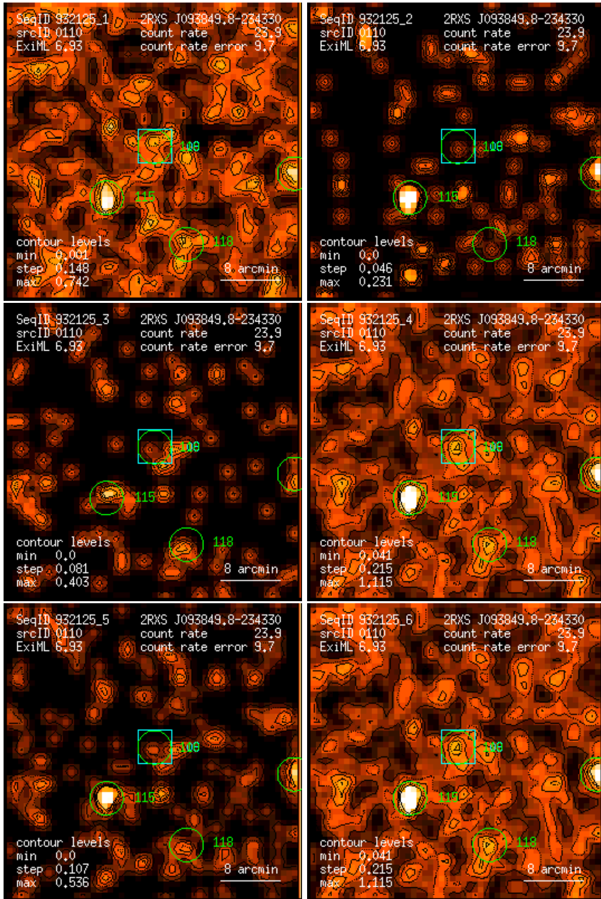
Figure 110: RASS 932125: detection 0110: band rate images, Gaussian filter: (1) PSPC channels 11 – 41, (2) 52 – 90, (3) 91 – 201, (4) 11 – 235, (5) 52 – 201, (6) 11 – 201. Broad band rates in counts/ks. Band rate contour levels in counts/ks/arcmin 2 .
