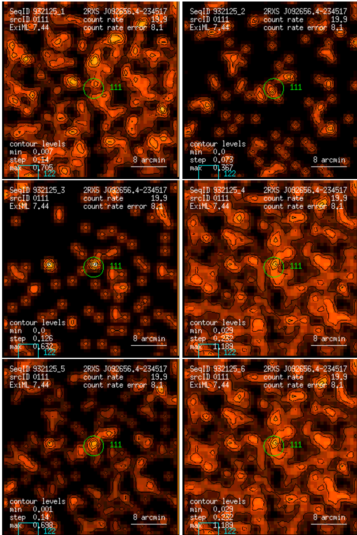
Figure 111: RASS 932125: detection 0111: band rate images, Gaussian filter: (1) PSPC channels 11 – 41, (2) 52 – 90, (3) 91 – 201, (4) 11 – 235, (5) 52 – 201, (6) 11 – 201. Broad band rates in counts/ks. Band rate contour levels in counts/ks/arcmin 2 .
