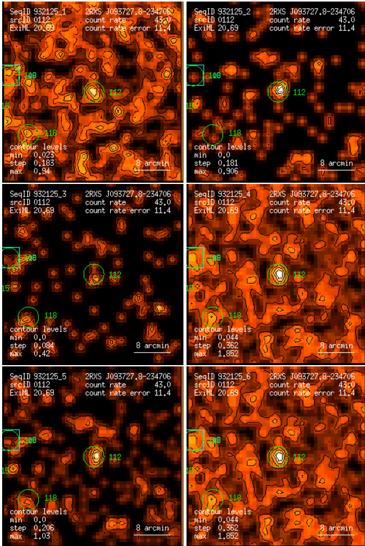
Figure 112: RASS 932125: detection 0112: band rate images, Gaussian filter: (1) PSPC channels 11 – 41, (2) 52 – 90, (3) 91 – 201, (4) 11 – 235, (5) 52 – 201, (6) 11 – 201. Broad band rates in counts/ks. Band rate contour levels in counts/ks/arcmin 2 .
