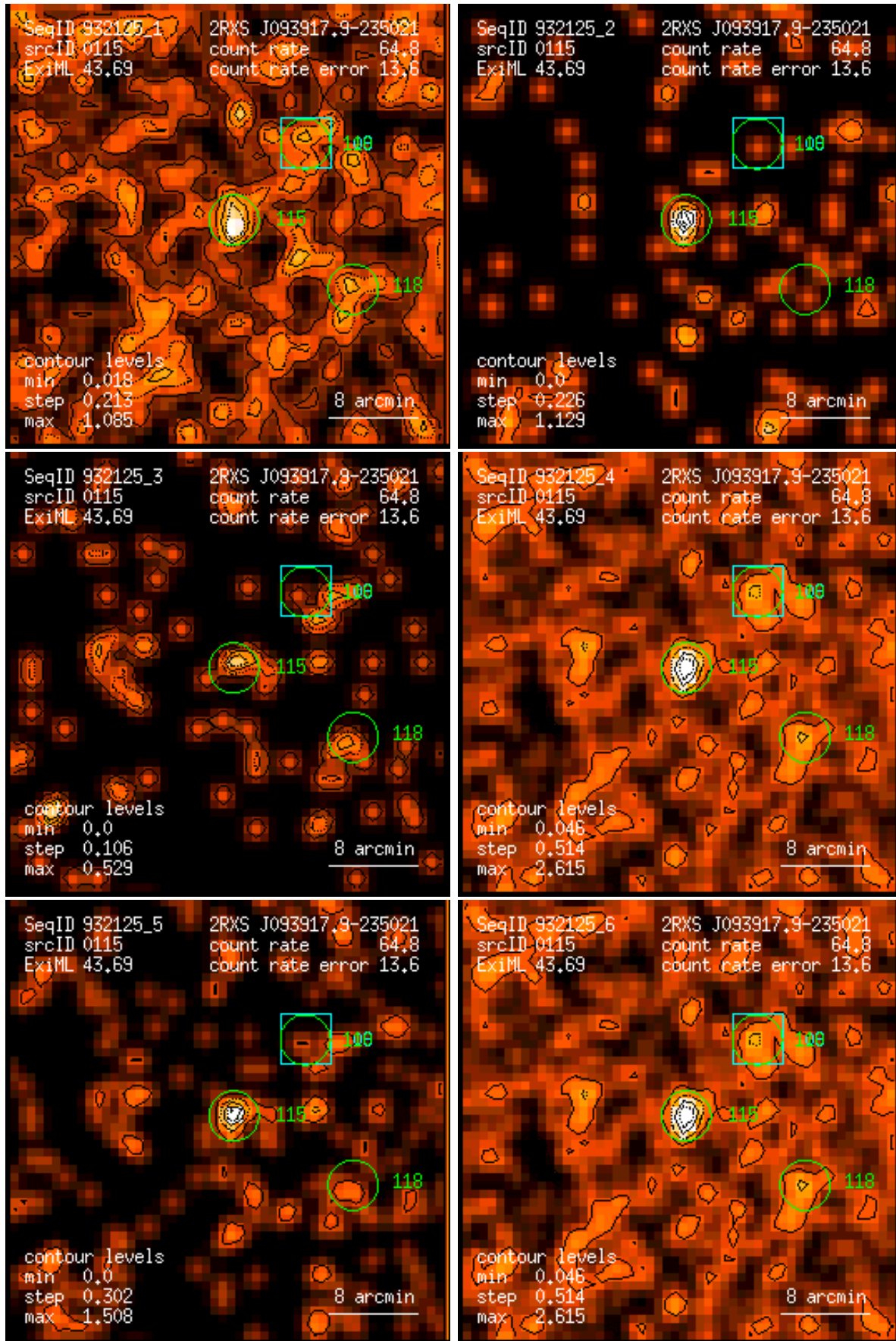
Figure 115: RASS 932125: detection 0115: band rate images, Gaussian filter: (1) PSPC channels 11 – 41, (2) 52 – 90, (3) 91 – 201, (4) 11 – 235, (5) 52 – 201, (6) 11 – 201. Broad band rates in counts/ks. Band rate contour levels in counts/ks/arcmin 2 .
