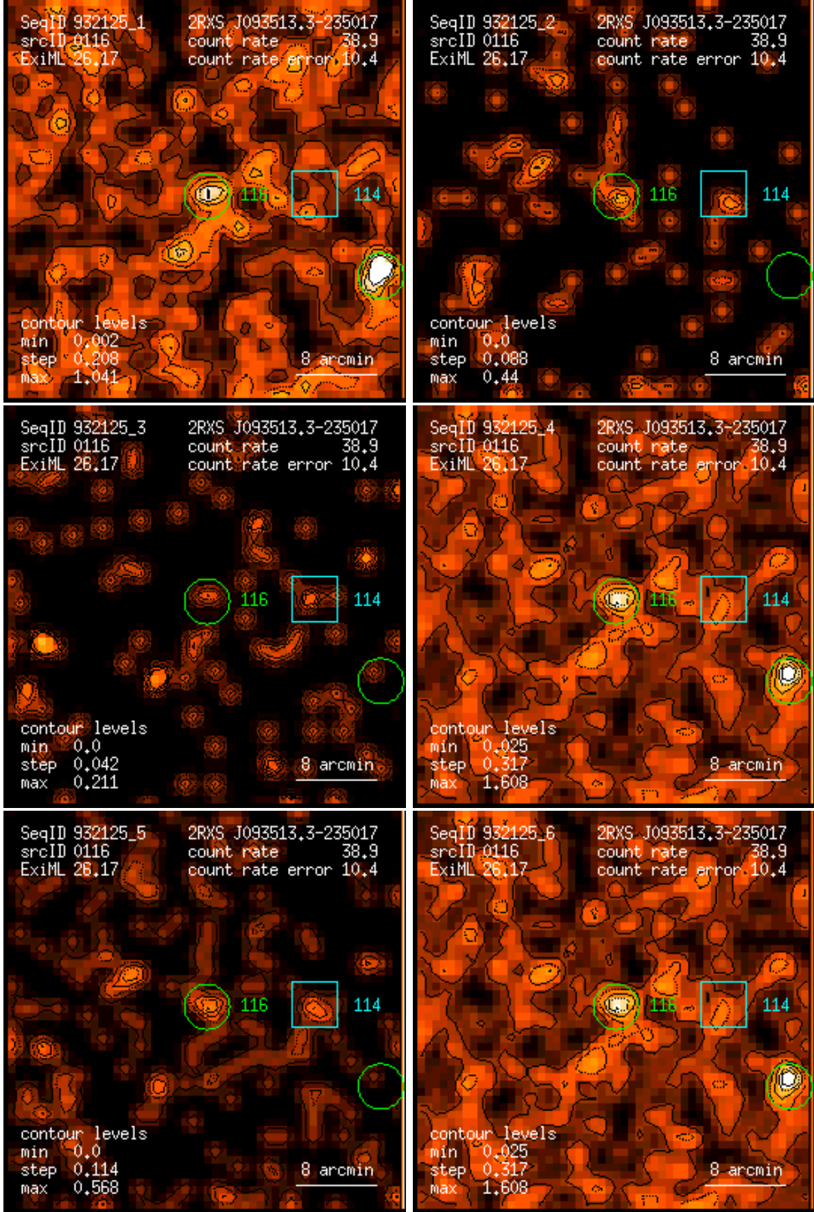
Figure 116: RASS 932125: detection 0116: band rate images, Gaussian filter: (1) PSPC channels 11 – 41, (2) 52 – 90, (3) 91 – 201, (4) 11 – 235, (5) 52 – 201, (6) 11 – 201. Broad band rates in counts/ks. Band rate contour levels in counts/ks/arcmin 2 .
