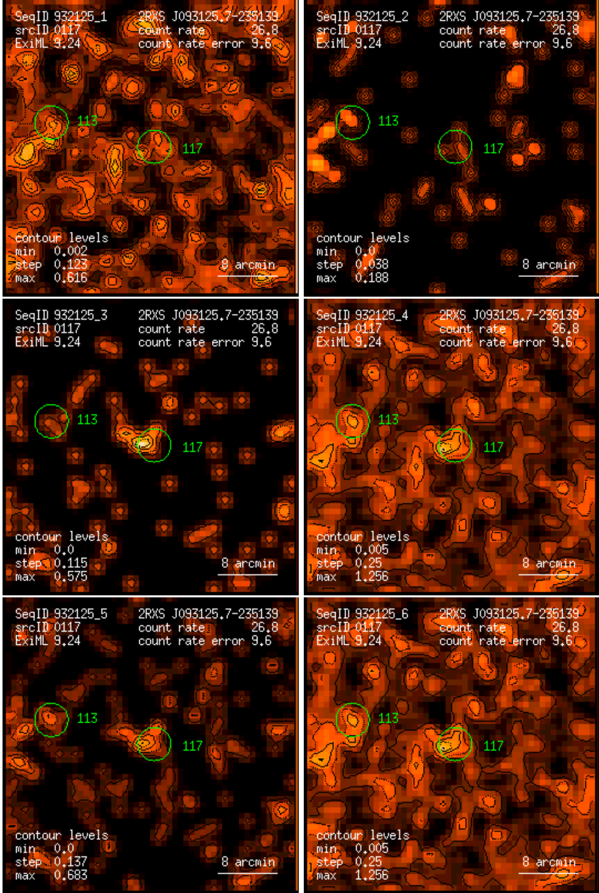
Figure 117: RASS 932125: detection 0117: band rate images, Gaussian filter: (1) PSPC channels 11 – 41, (2) 52 – 90, (3) 91 – 201, (4) 11 – 235, (5) 52 – 201, (6) 11 – 201. Broad band rates in counts/ks. Band rate contour levels in counts/ks/arcmin 2 .
