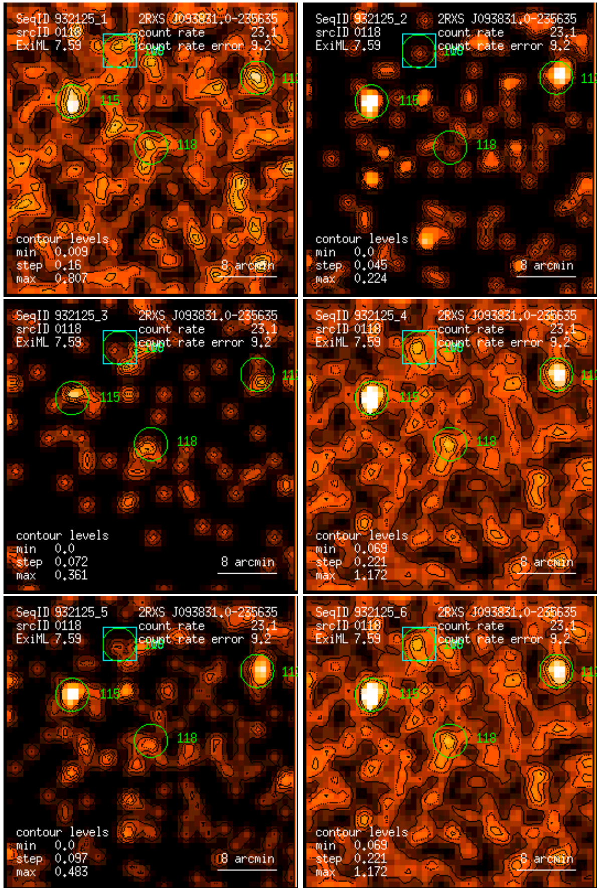
Figure 118: RASS 932125: detection 0118: band rate images, Gaussian filter: (1) PSPC channels 11 – 41, (2) 52 – 90, (3) 91 – 201, (4) 11 – 235, (5) 52 – 201, (6) 11 – 201. Broad band rates in counts/ks. Band rate contour levels in counts/ks/arcmin 2 .
