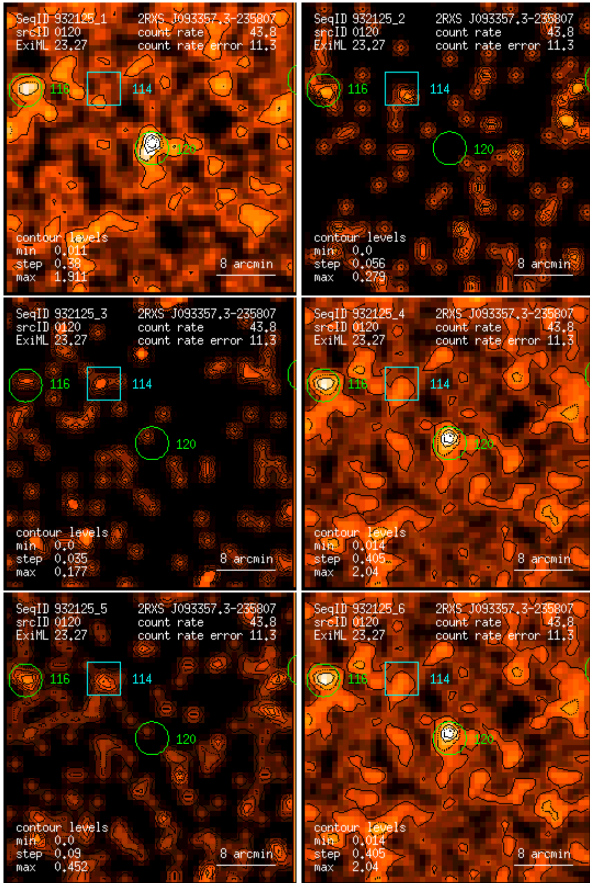
Figure 120: RASS 932125: detection 0120: band rate images, Gaussian filter: (1) PSPC channels 11 – 41, (2) 52 – 90, (3) 91 – 201, (4) 11 – 235, (5) 52 – 201, (6) 11 – 201. Broad band rates in counts/ks. Band rate contour levels in counts/ks/arcmin 2 .
