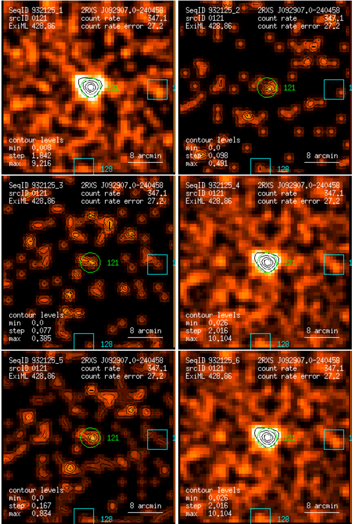
Figure 121: RASS 932125: detection 0121: band rate images, Gaussian filter: (1) PSPPC channels 11 – 41, (2) 52 – 90, (3) 91 – 201, (4) 11 – 235, (5) 52 – 201, (6) 11 – 201. Broad band rates in counts/ks. Band rate contour levels in counts/ks/arcmin 2 .
