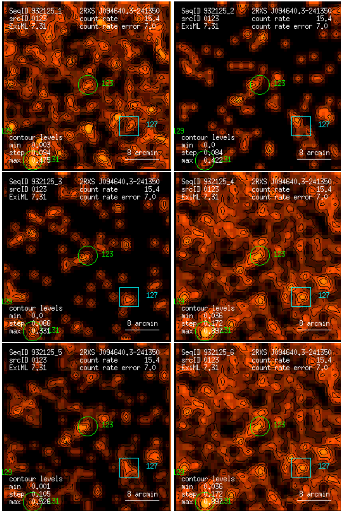
Figure 123: RASS 932125: detection 0123: band rate images, Gaussian filter: (1) PSPC channels 11 – 41, (2) 52 – 90, (3) 91 – 201, (4) 11 – 235, (5) 52 – 201, (6) 11 – 201. Broad band rates in counts/ks. Band rate contour levels in counts/ks/arcmin 2 .
